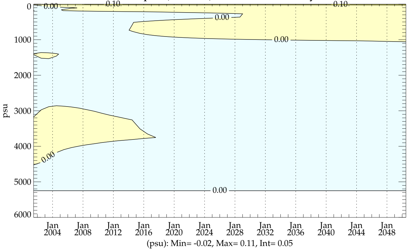
thres05 (20010101 - 20501231) - Levitus ZT-plot (0-6000m) Global Mean Salinity
