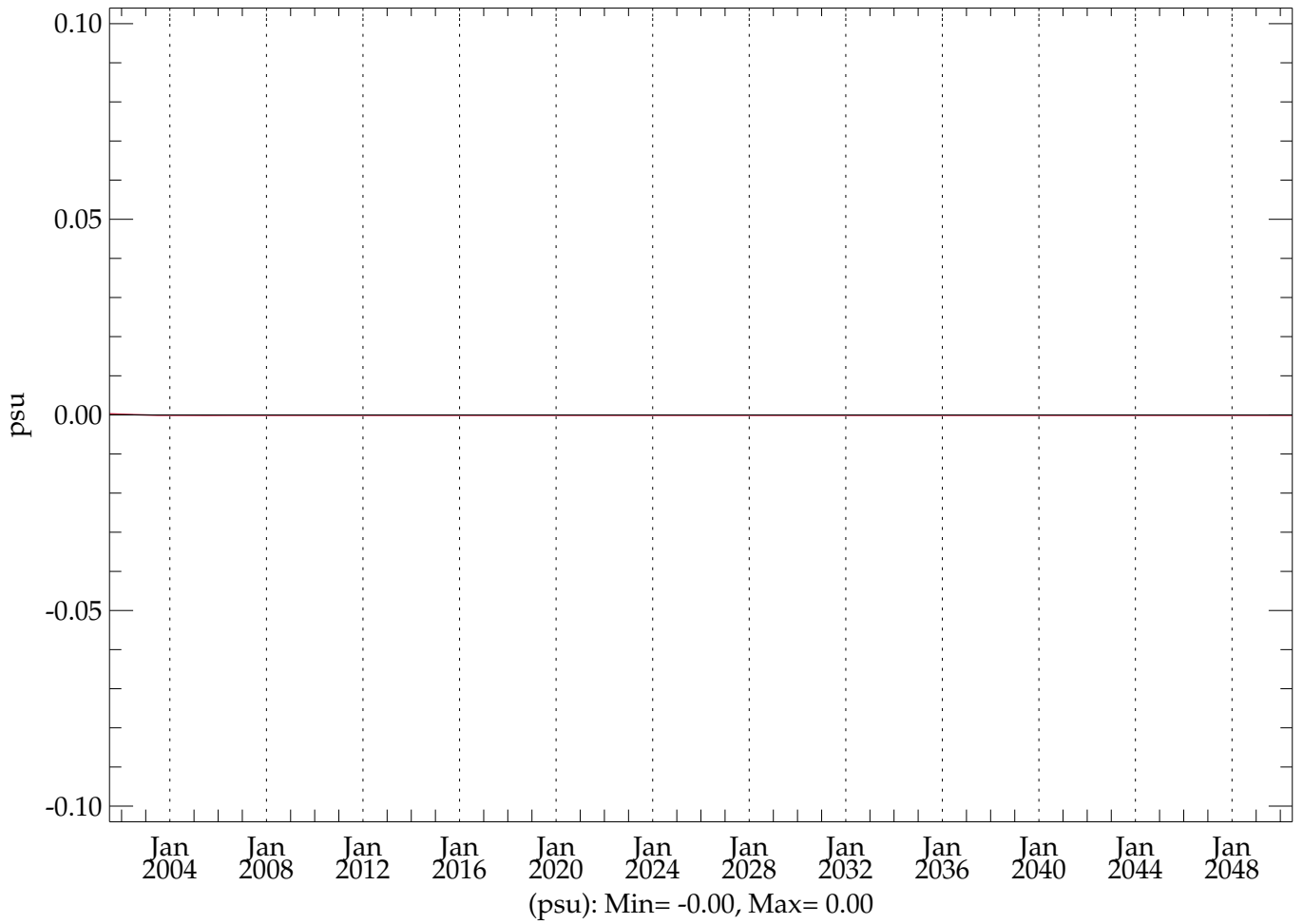
thres05 - testht (20010101 - 20501231) ZT-plot (0-6000m) Global Mean Salinity
