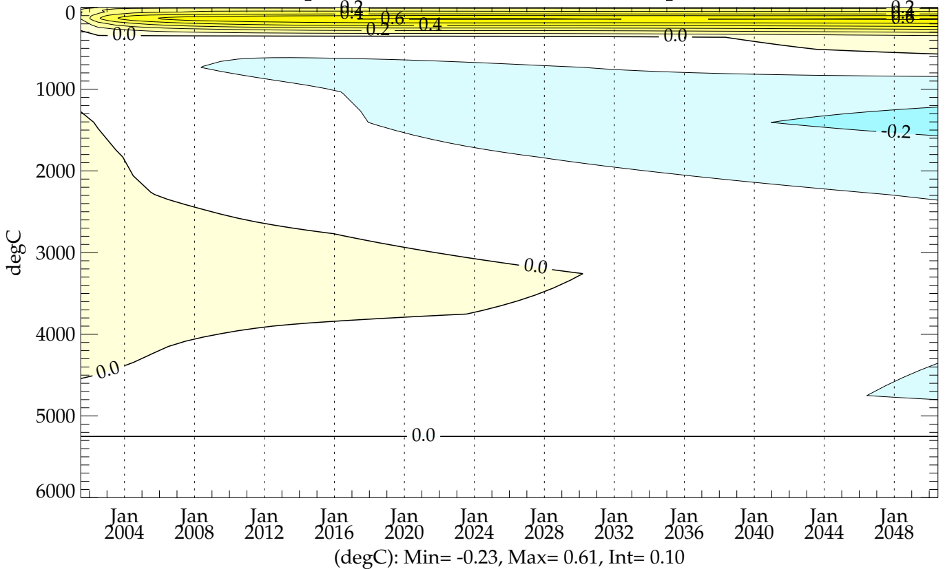
thres05 (20010101 - 20501231) - Levitus ZT-plot (0-6000m) Global Mean Temperature
