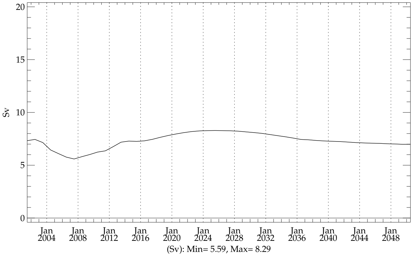
thres05 (20010101 - 20501231) Max AntArctic Bottom Water between 80S and 65S (20010101 - 20501231)
