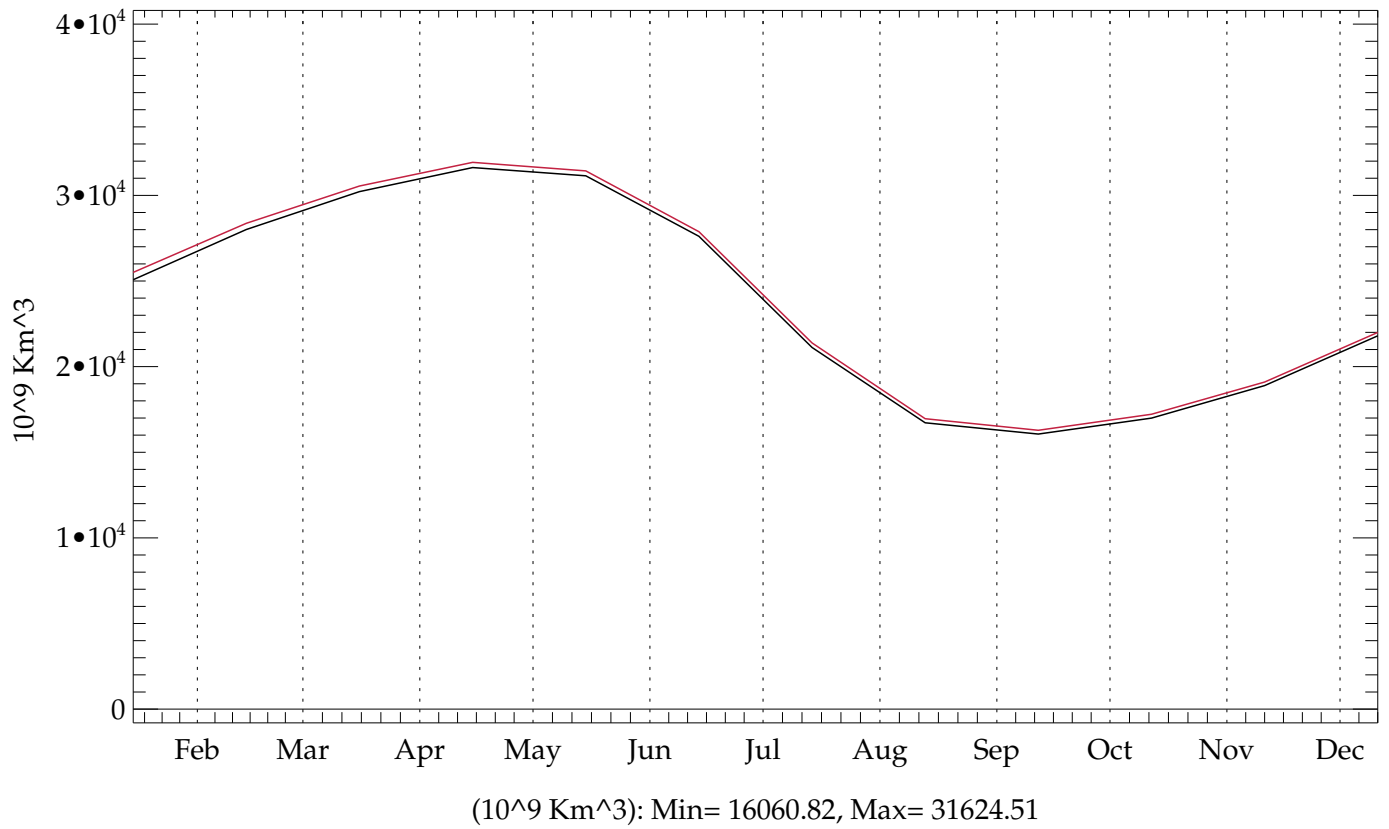
Northern Hemisphere thres05 (BLACK) - testht (RED) (20010101 - 20501231) Global Annual Mean Ice Volume (BLACK)
