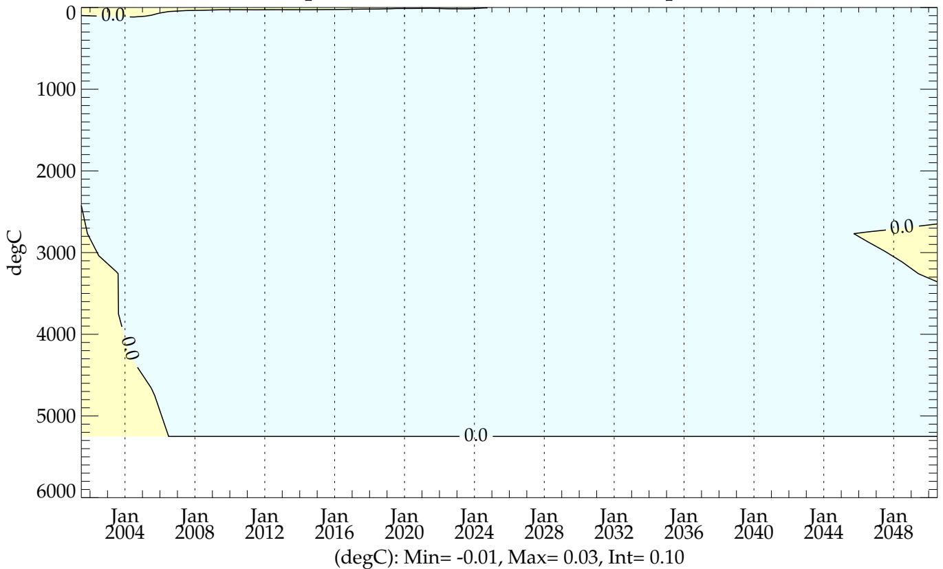
thres05 - testht (20010101 - 20501231) ZT-plot (0-6000m) Global Mean Temperature
