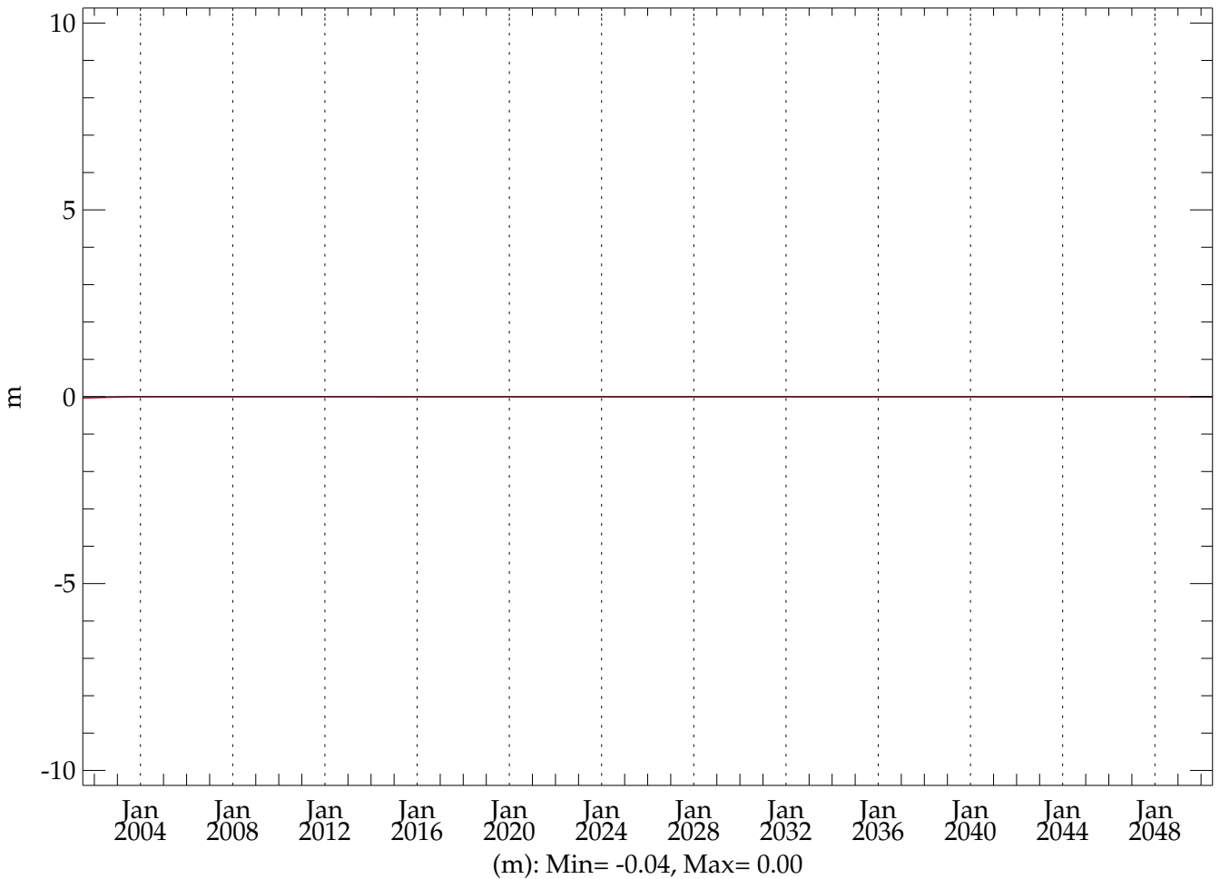
thres05 (BLACK) - testht (RED) (20010101 - 20501231) Global Mean SSH
