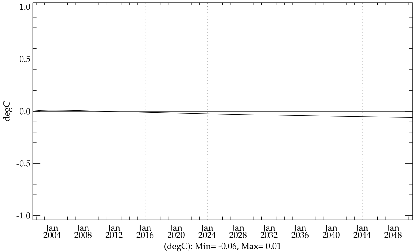
thres05 (20010101 - 20501231) - Levitus Global Mean Temperature
