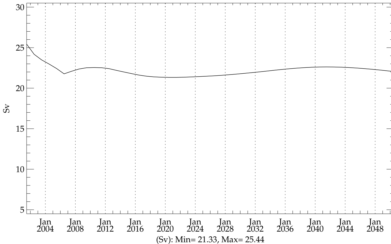
thres05 (20010101 - 20501231) Max AntArctic Bottom Cell between 65S and 30N (20010101 - 20501231)
