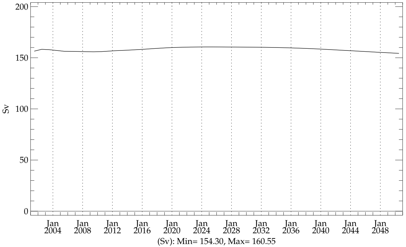
thres05 (20010101 - 20501231) Drake Transport
