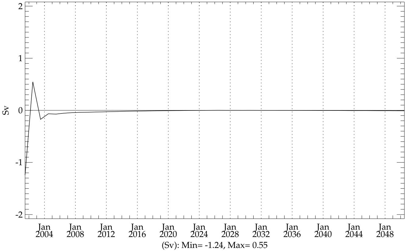
thres05 (20010101 - 20501231) Global Mean EMP
