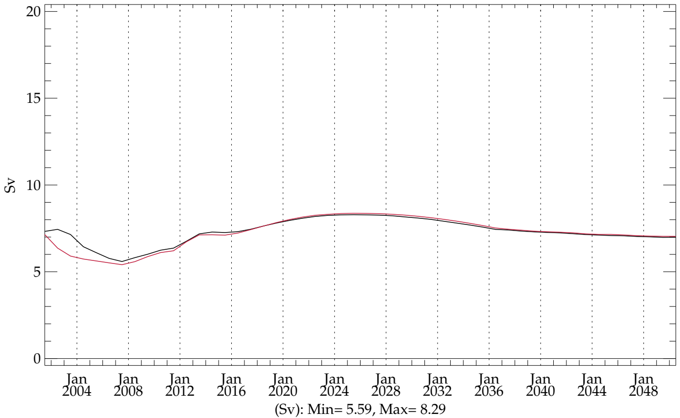
thres05 (BLACK) - testht (RED) (20010101 - 20501231) Max AntArctic Bottom Water between 80S and 65S
