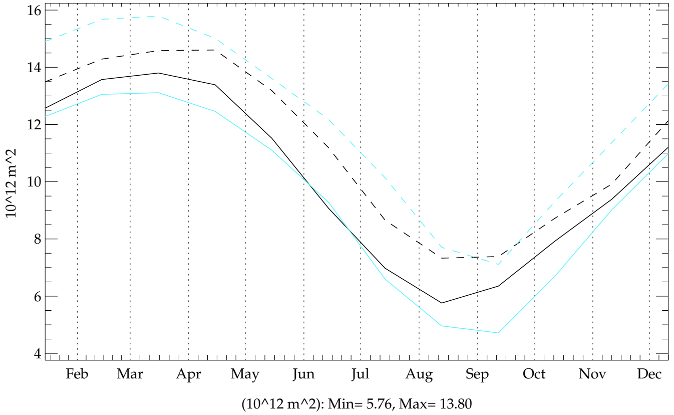
Southern Hemisphere thres05 (BLACK) (20010101 - 20501231) OBSERVATION (light blue) Global Annual Mean Ice Area (CONTINUOUS) and Extend minus 15% (DASHED)
