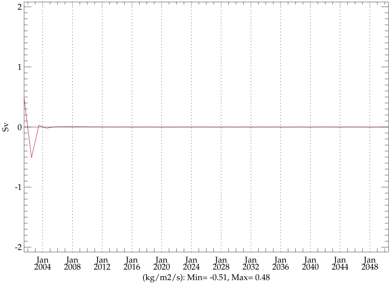
thres05 (BLACK) - testht (RED) (20010101 - 20501231) Global Mean EMP
