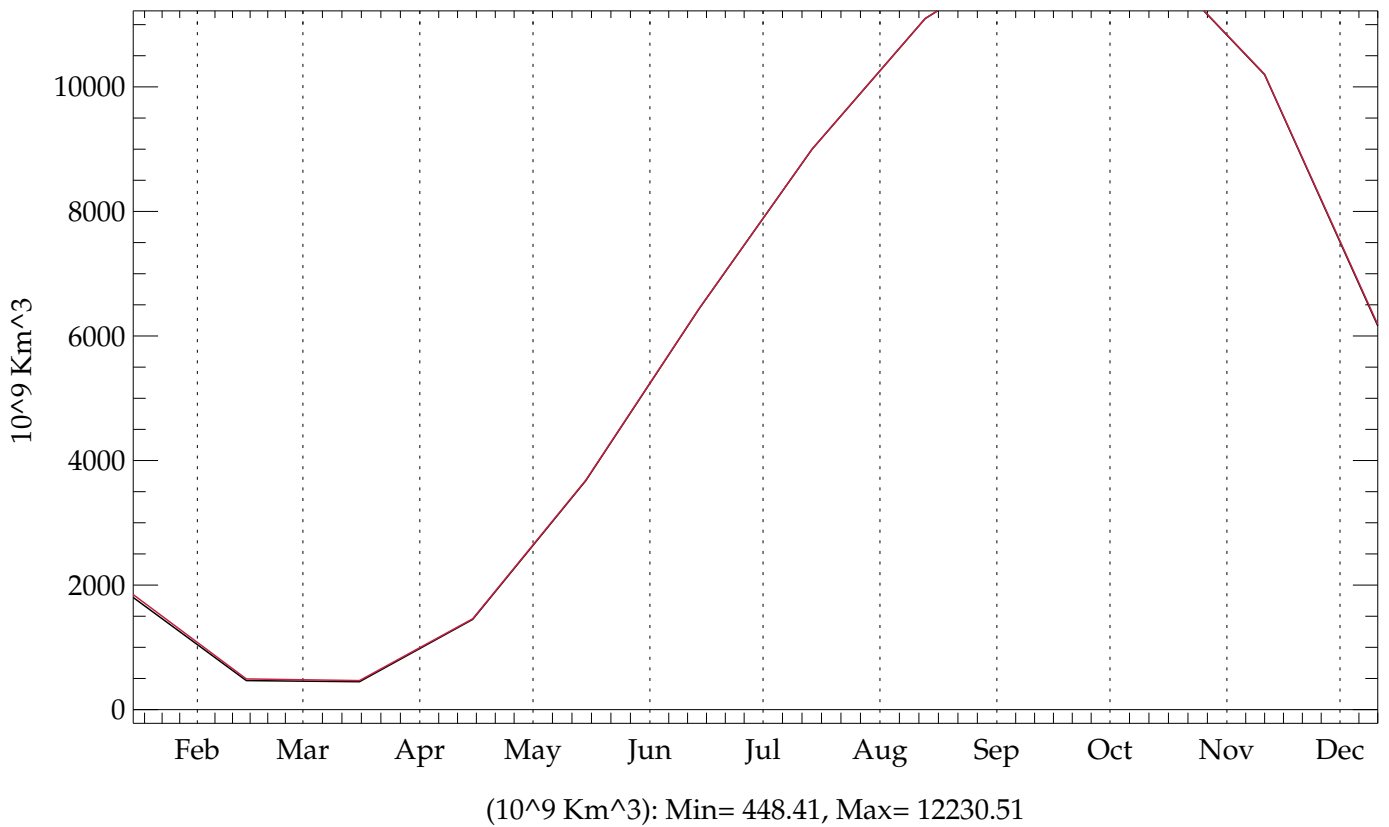
Southern Hemisphere thres05 (BLACK) - testht (RED) (20010101 - 20501231) Global Annual Mean Ice Volume
