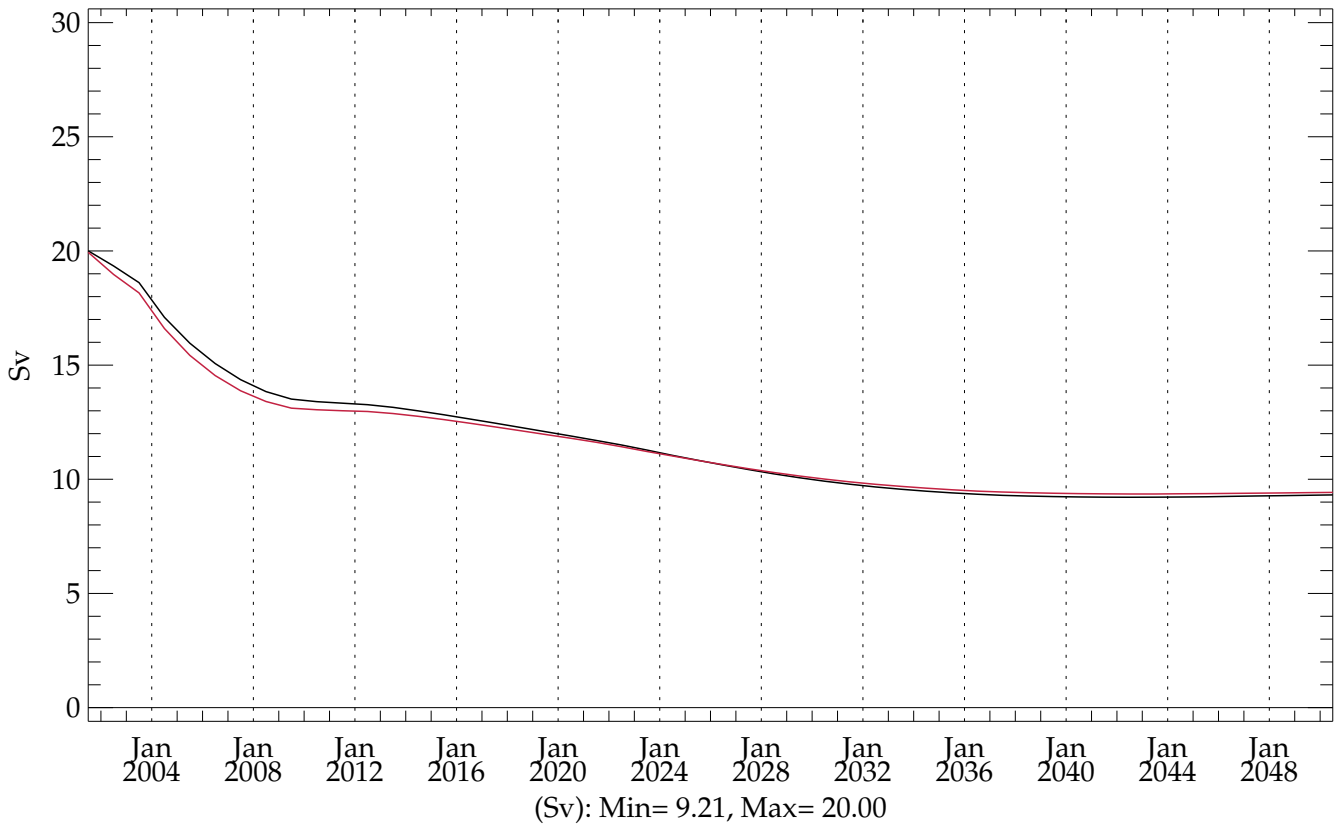
thres05 (BLACK) - testht (RED) (20010101 - 20501231) Max Atlantic MOC between 40N and 50N
