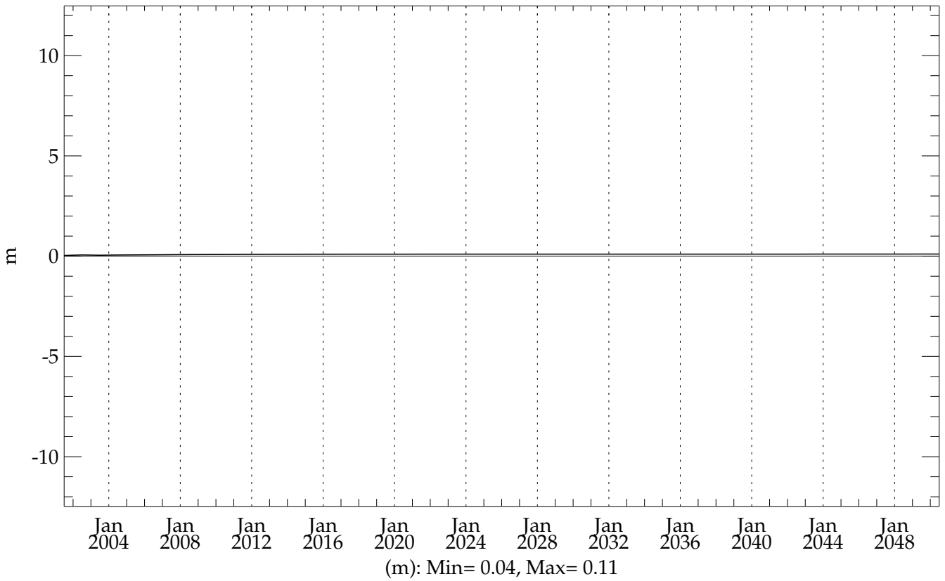
thres05 (20010101 - 20501231) Global Mean SSH
