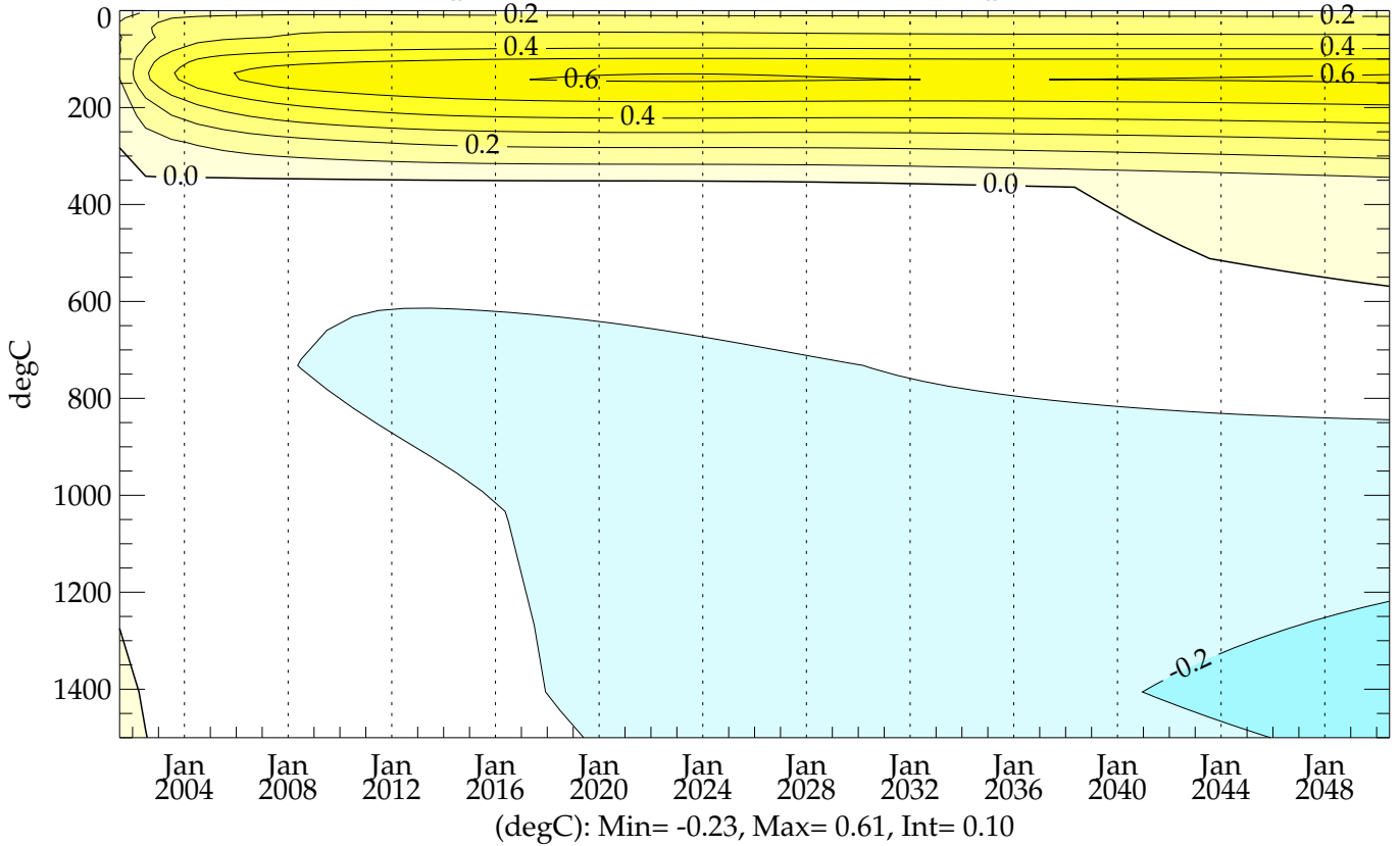
thres05 (20010101 - 20501231) - Levitus ZT-plot (0-1500m) Global Mean Temperature
