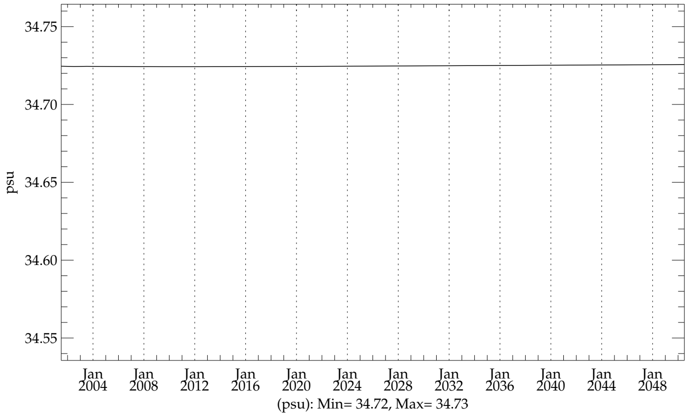
thres05 (20010101 - 20501231) Global Mean Salinity
