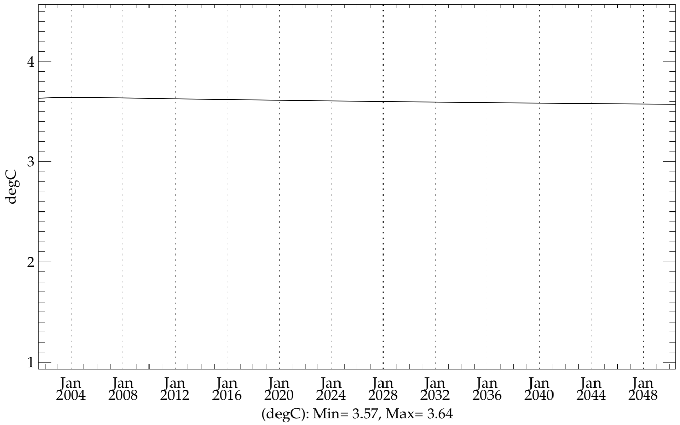
thres05 (20010101 - 20501231) Global Mean Temperature
