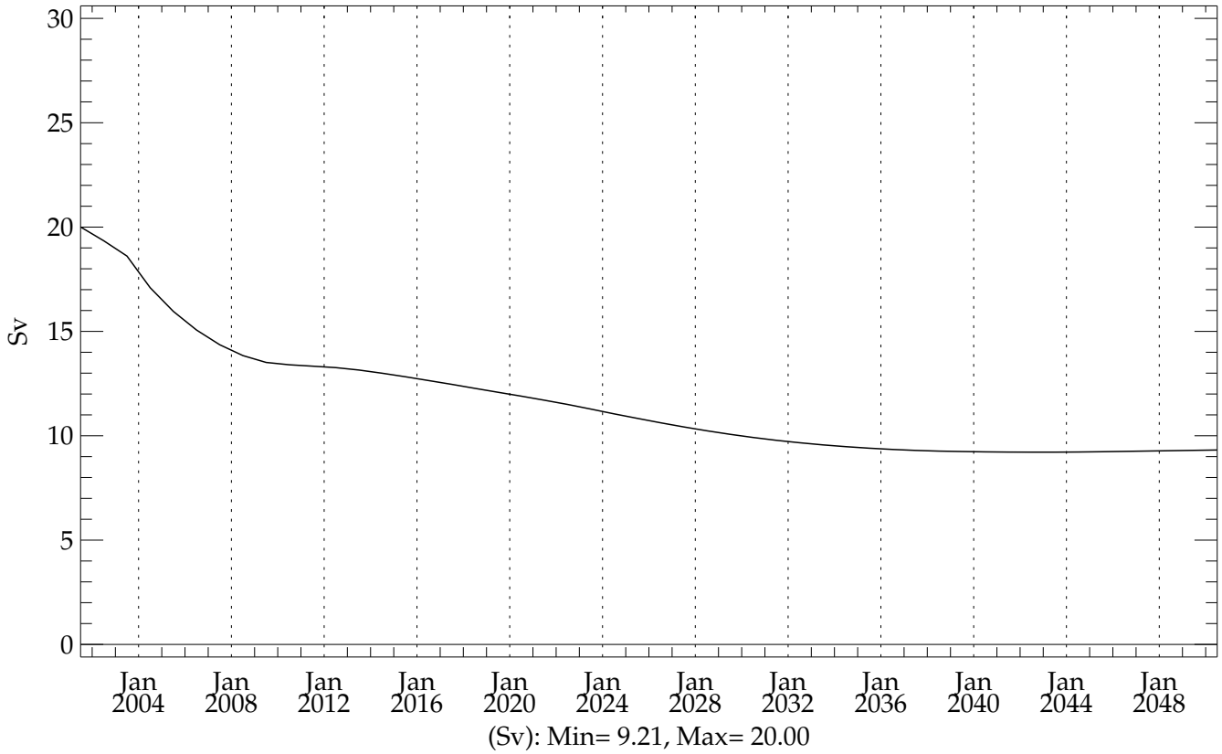
thres05 (20010101 - 20501231) Max Atlantic MOC between 40N and 50N
