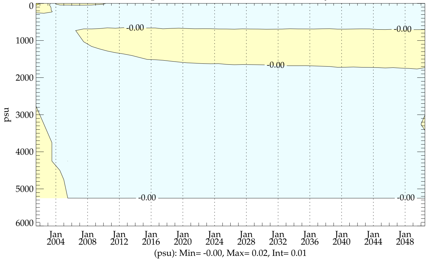
thres05 - testht (20010101 - 20501231) ZT-plot (0-6000m) Global Mean Salinity
