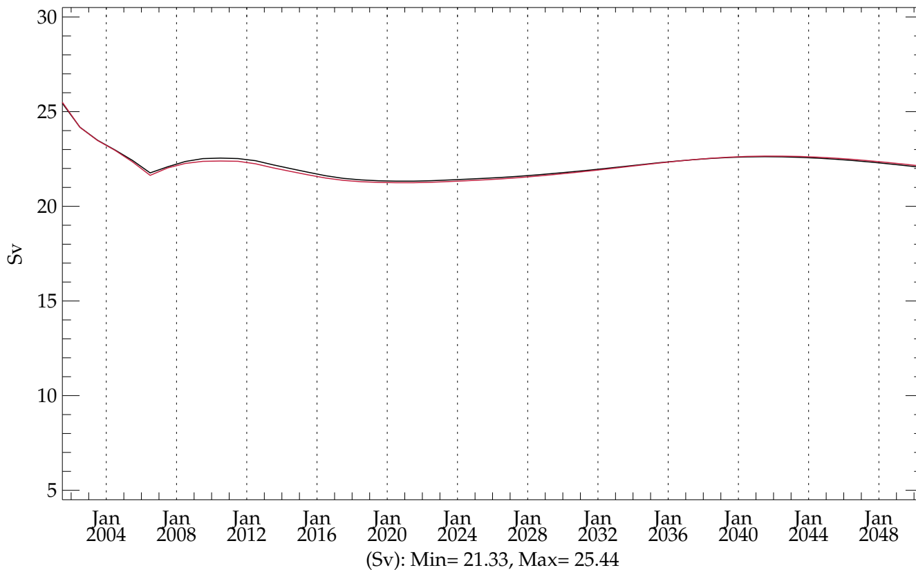
thres05 (BLACK) - testht (RED) (20010101 - 20501231) Max AntArctic Bottom Cell between 65S and 30N
