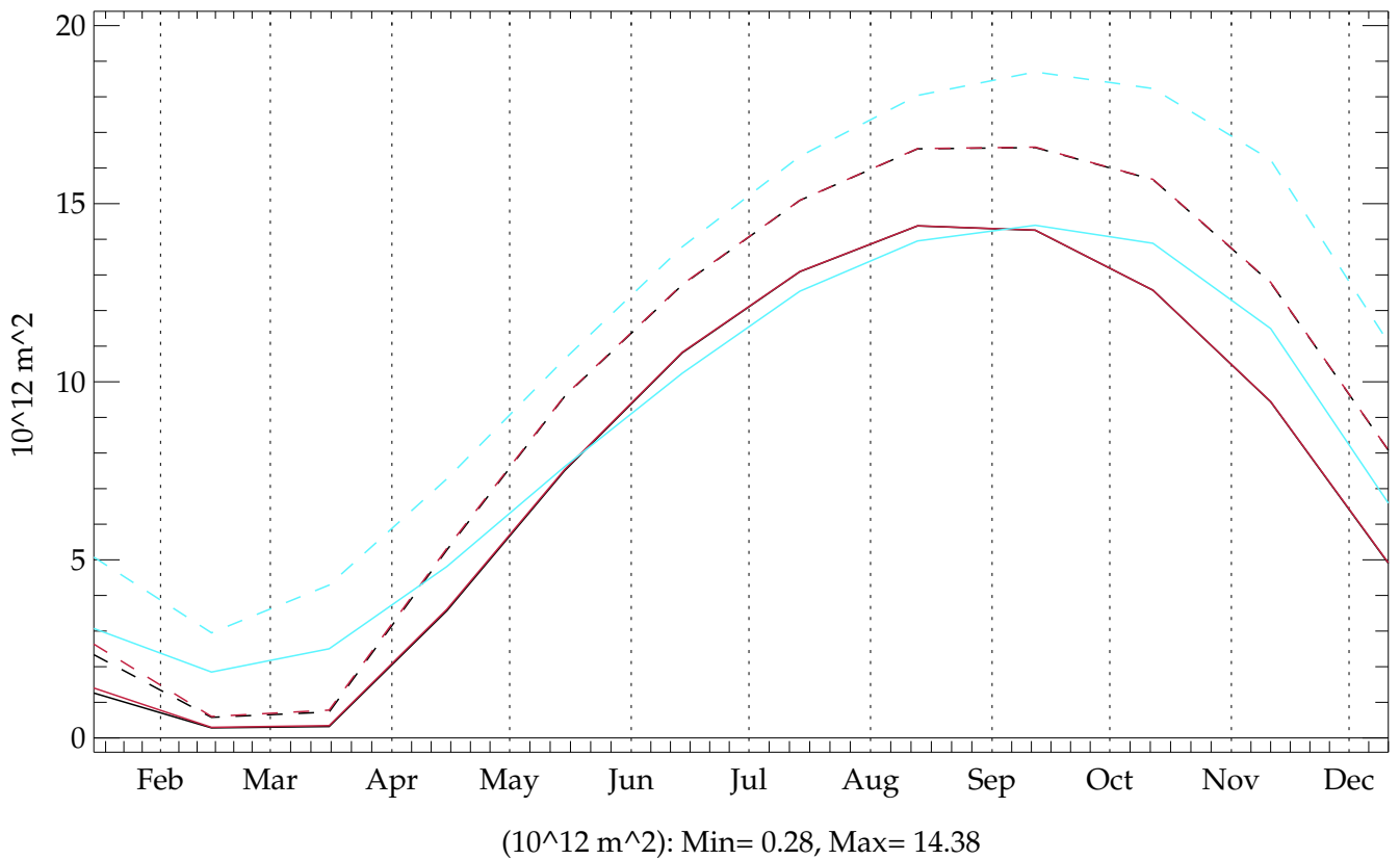
Southern Hemisphere thres05 (BLACK) - testht (RED) (20010101 - 20501231) OBSERVATION (light blue) Global Annual Mean Ice Area (CONTINUOUS) and Extend minus 15% (DASHED)
