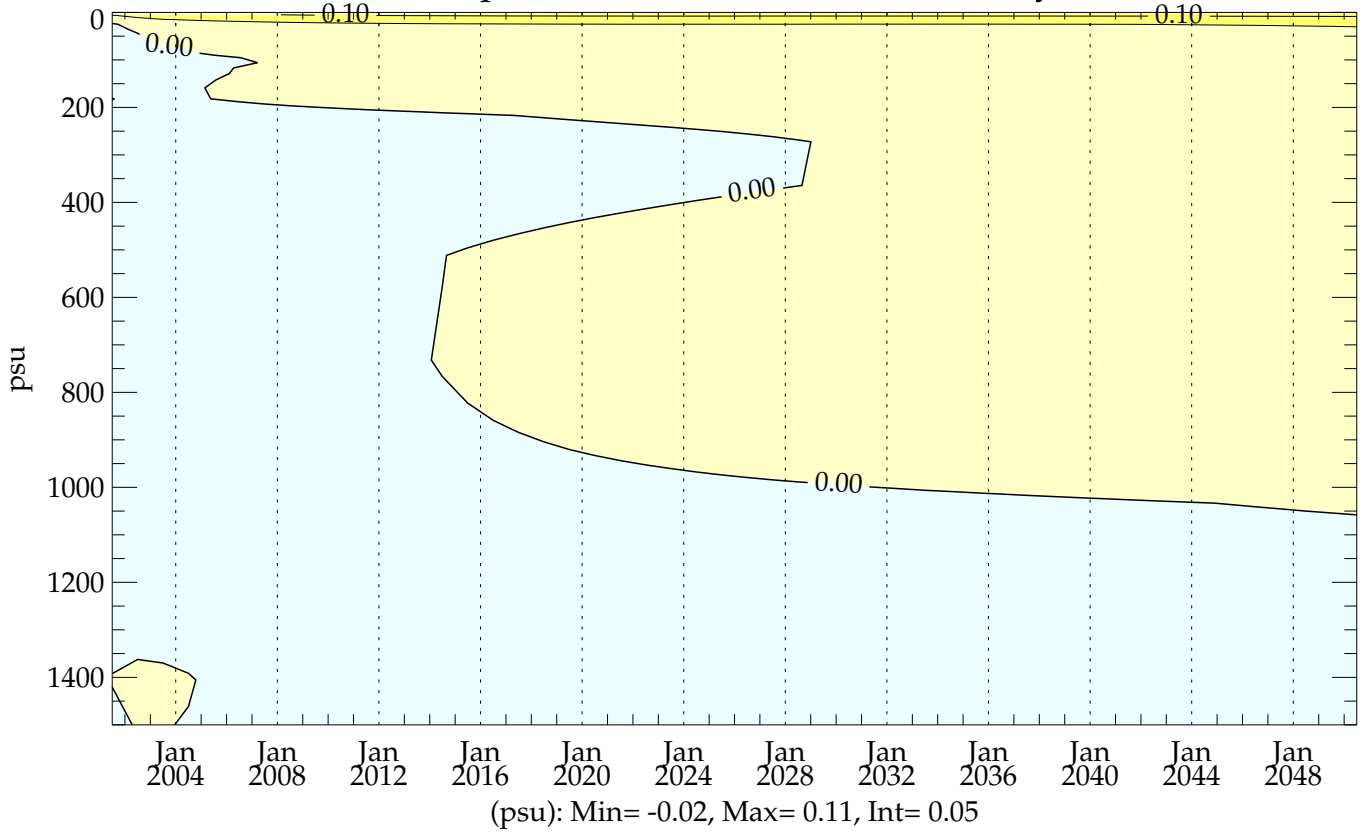
thres05 (20010101 - 20501231) - Levitus ZT-plot (0-1500m) Global Mean Salinity
