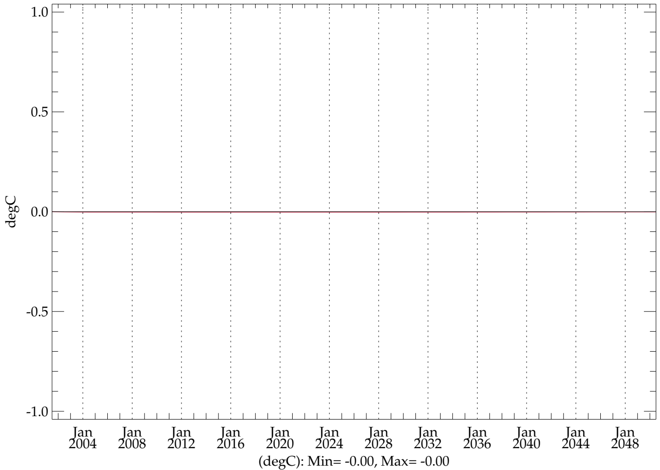
thres05 - testht (20010101 - 20501231) ZT-plot (0-6000m) Global Mean Temperature
