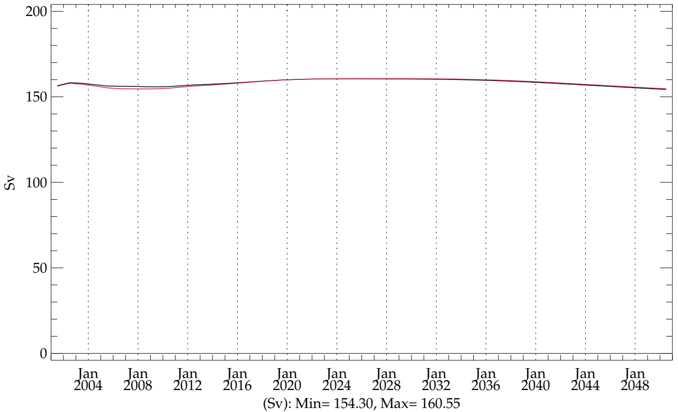
thres05 (BLACK) - testht (RED) (20010101 - 20501231) Drake Transport
