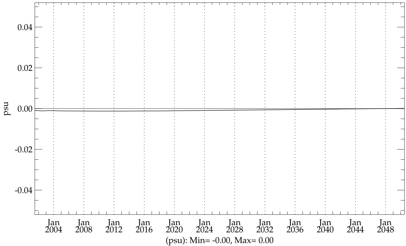
thres05 (20010101 - 20501231) - Levitus Global Mean Salinity
