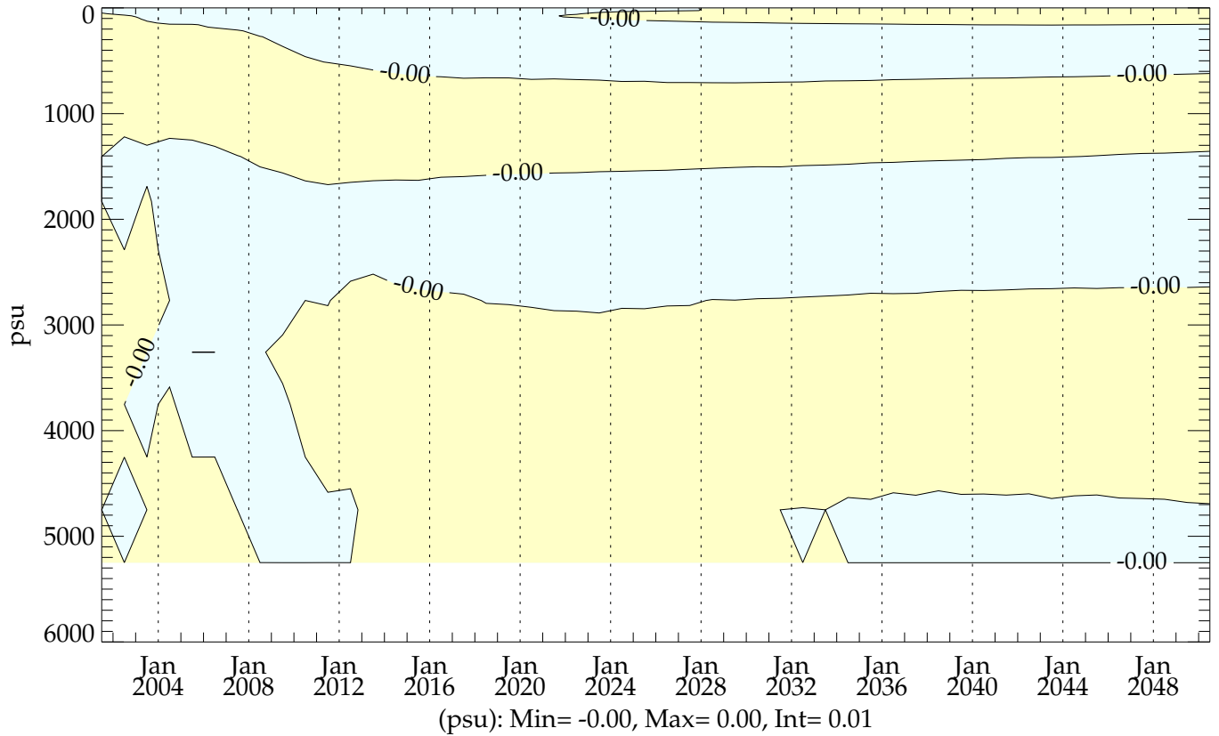
pstar4 - testht (20010101 - 20501231) ZT-plot (0-6000m) Global Mean Salinity
