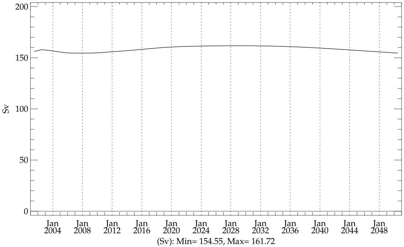
pstar4 (20010101 - 20501231) Drake Transport
