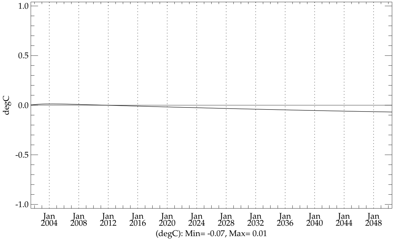
pstar4 (20010101 - 20501231) - Levitus Global Mean Temperature
