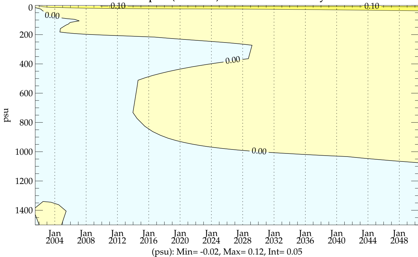
pstar4 (20010101 - 20501231) - Levitus ZT-plot (0-1500m) Global Mean Salinity
