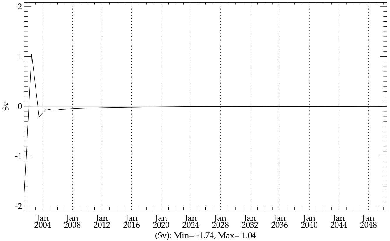
pstar4 (20010101 - 20501231) Global Mean EMP
