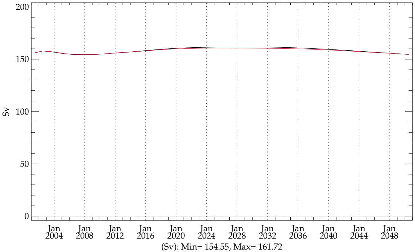
pstar4 (BLACK) - testht (RED) (20010101 - 20501231) Drake Transport
