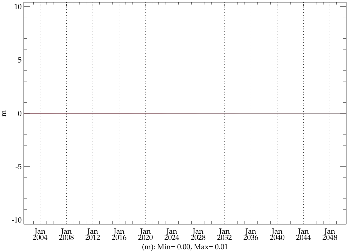
pstar4 (BLACK) - testht (RED) (20010101 - 20501231) Global Mean SSH
