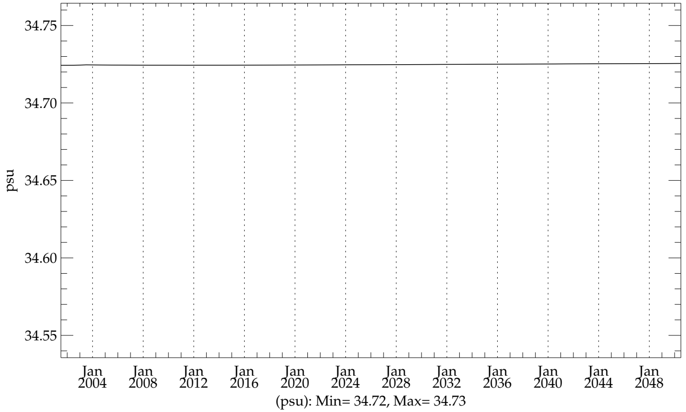
pstar4 (20010101 - 20501231) Global Mean Salinity
