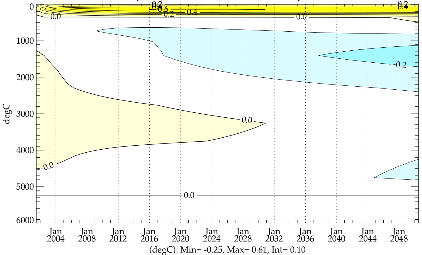
pstar4 (20010101 - 20501231) - Levitus ZT-plot (0-6000m) Global Mean Temperature
