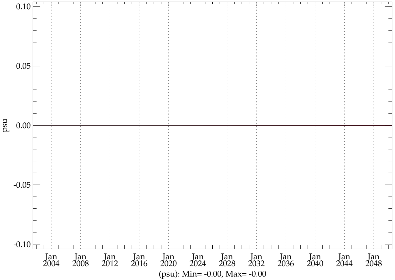
pstar4 - testht (20010101 - 20501231) ZT-plot (0-6000m) Global Mean Salinity
