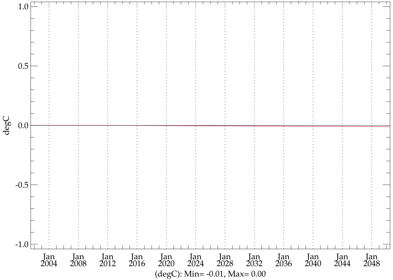
pstar4 - testht (20010101 - 20501231) ZT-plot (0-6000m) Global Mean Temperature
