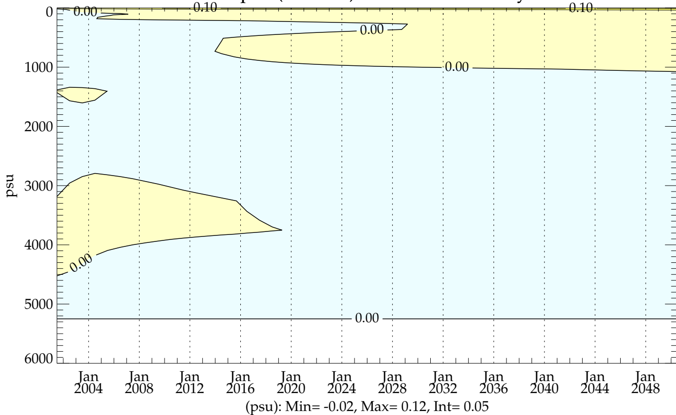
pstar4 (20010101 - 20501231) - Levitus ZT-plot (0-6000m) Global Mean Salinity
