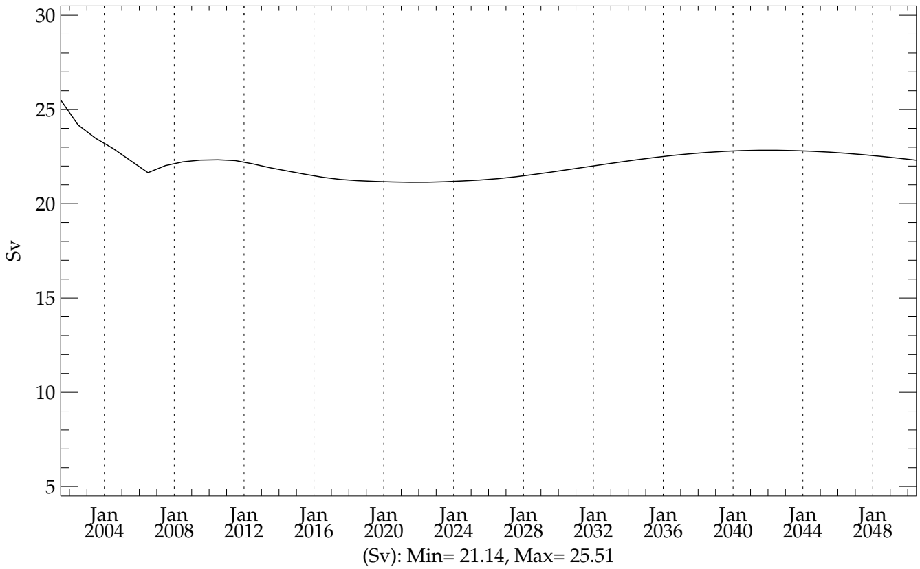
pstar4 (20010101 - 20501231) Max AntArctic Bottom Cell between 65S and 30N (20010101 - 20501231)
