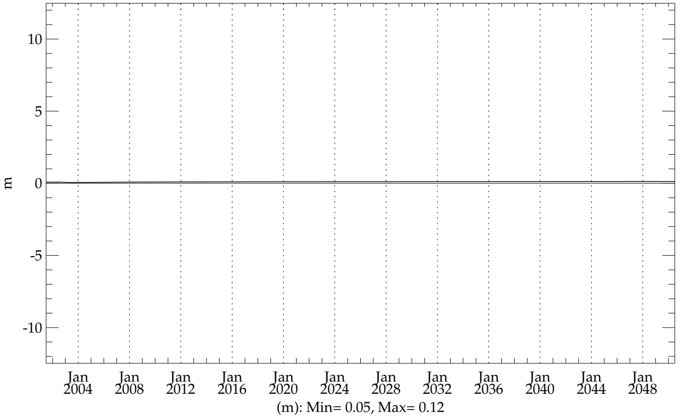
pstar4 (20010101 - 20501231) Global Mean SSH
