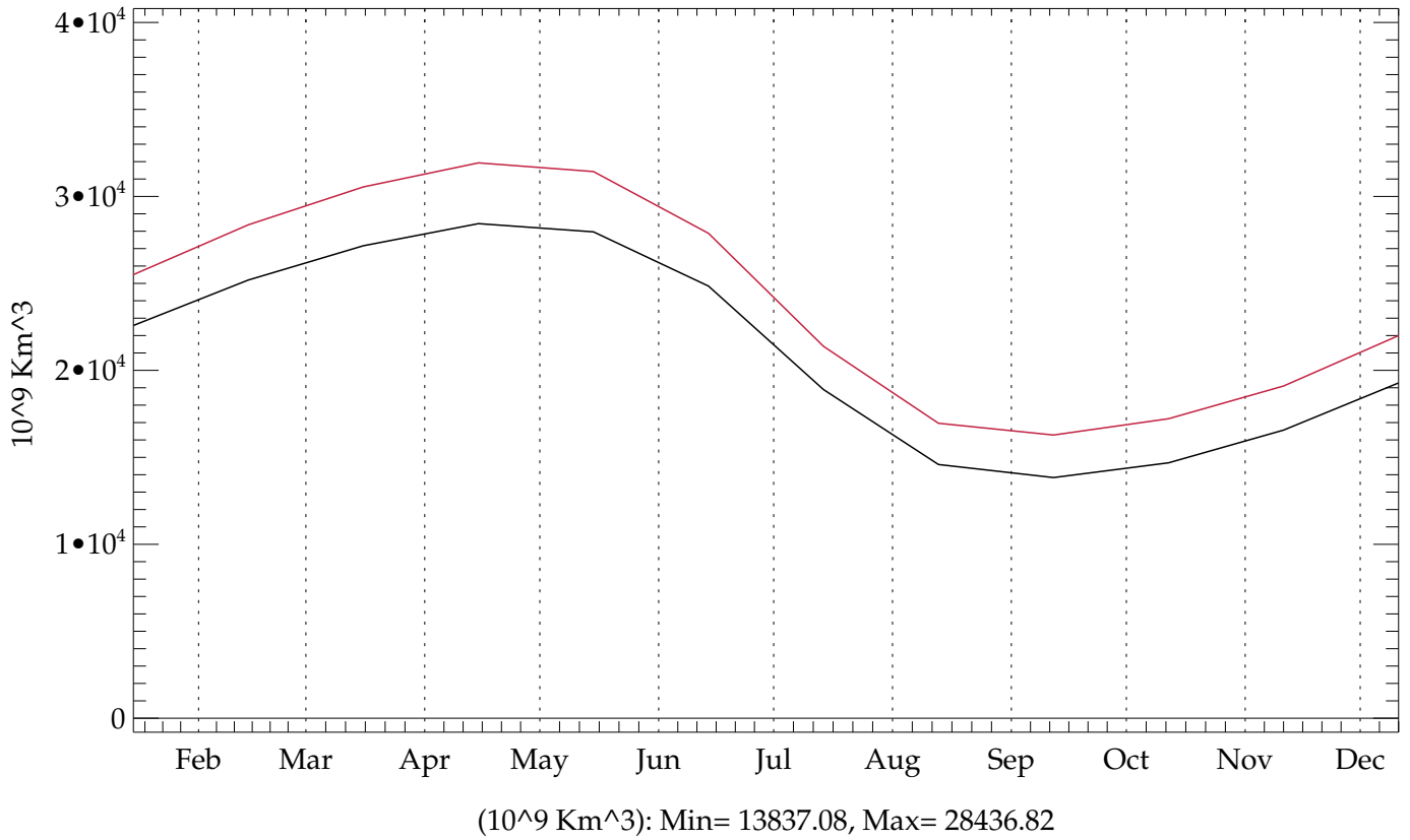
Northern Hemisphere pstar4 (BLACK) - testht (RED) (20010101 - 20501231) Global Annual Mean Ice Volume (BLACK)
