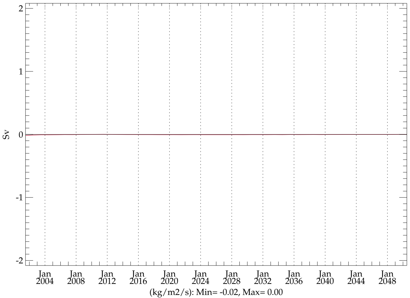
pstar4 (BLACK) - testht (RED) (20010101 - 20501231) Global Mean EMP
