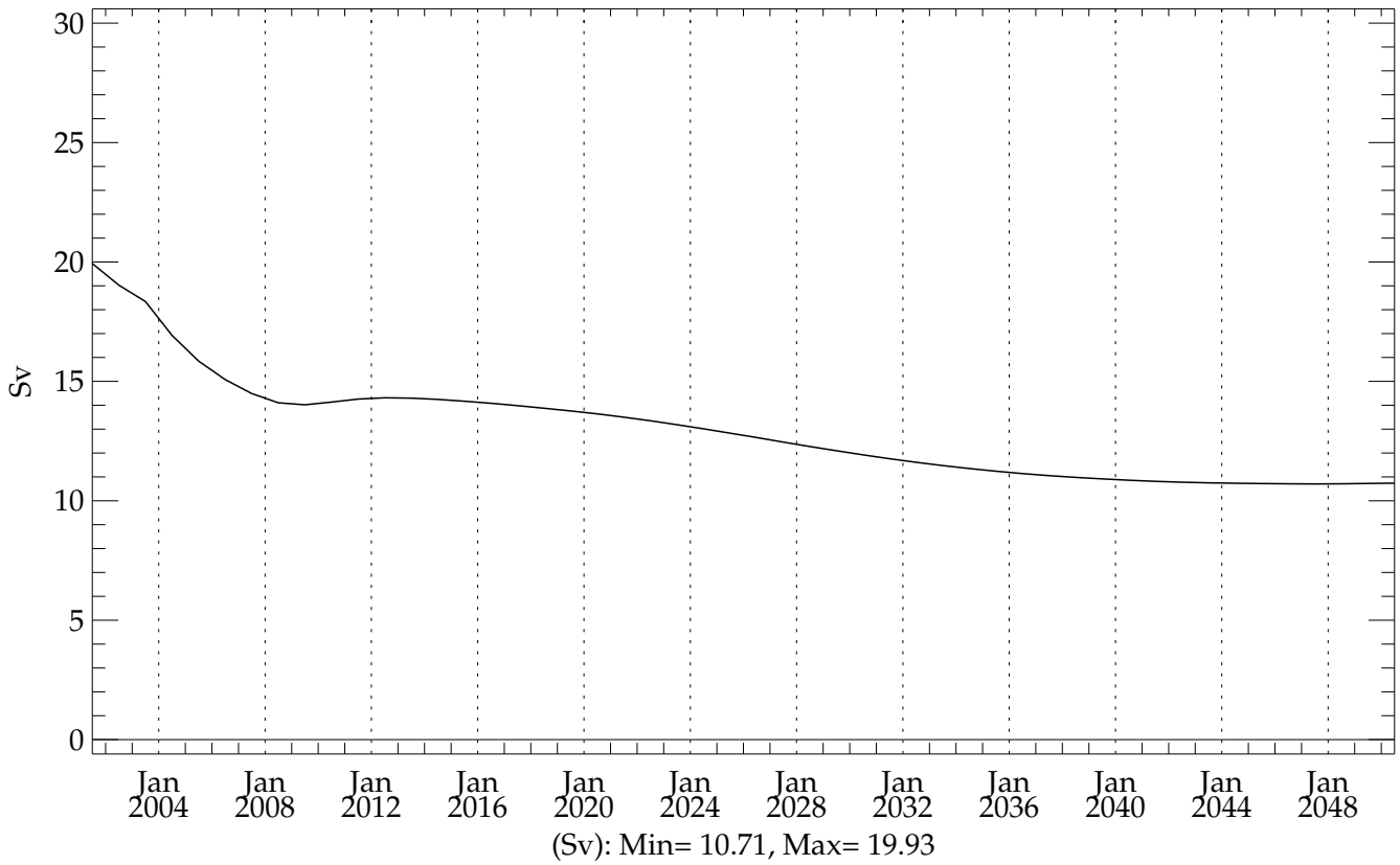
pstar4 (20010101 - 20501231) Max Atlantic MOC between 40N and 50N
