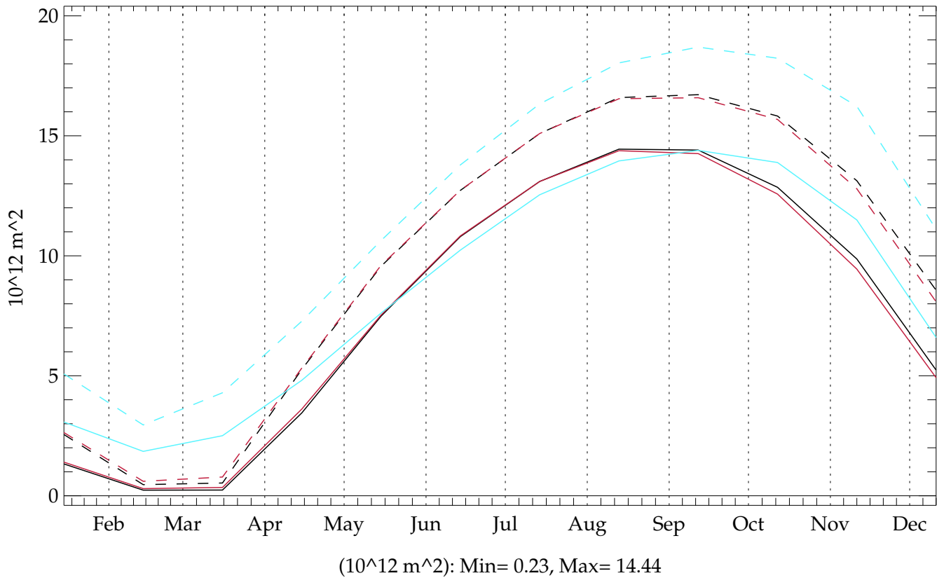
Southern Hemisphere pstar4 (BLACK) - testht (RED) (20010101 - 20501231) OBSERVATION (light blue) Global Annual Mean Ice Area (CONTINUOUS) and Extend minus 15% (DASHED)
