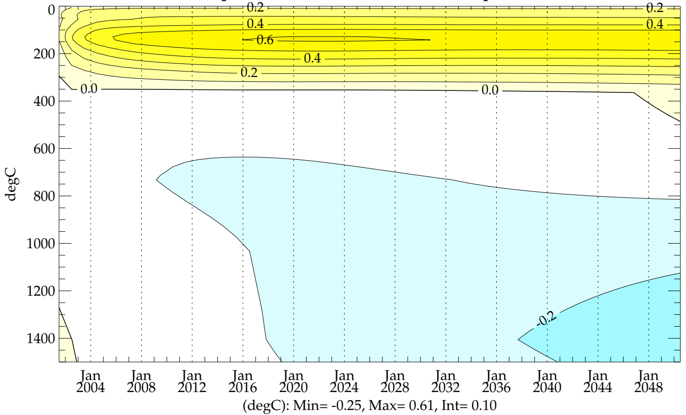
pstar4 (20010101 - 20501231) - Levitus ZT-plot (0-1500m) Global Mean Temperature
