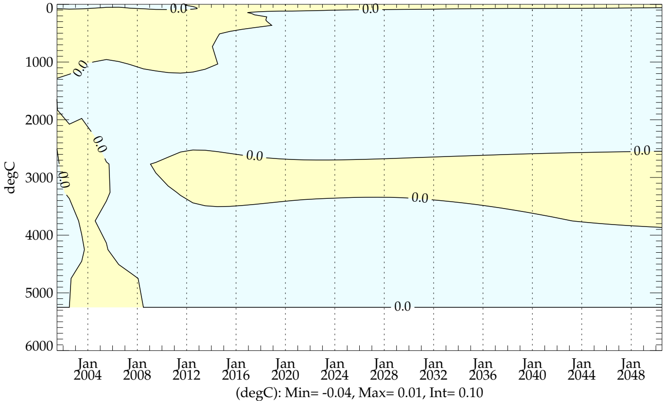
pstar4 - testht (20010101 - 20501231) ZT-plot (0-6000m) Global Mean Temperature
