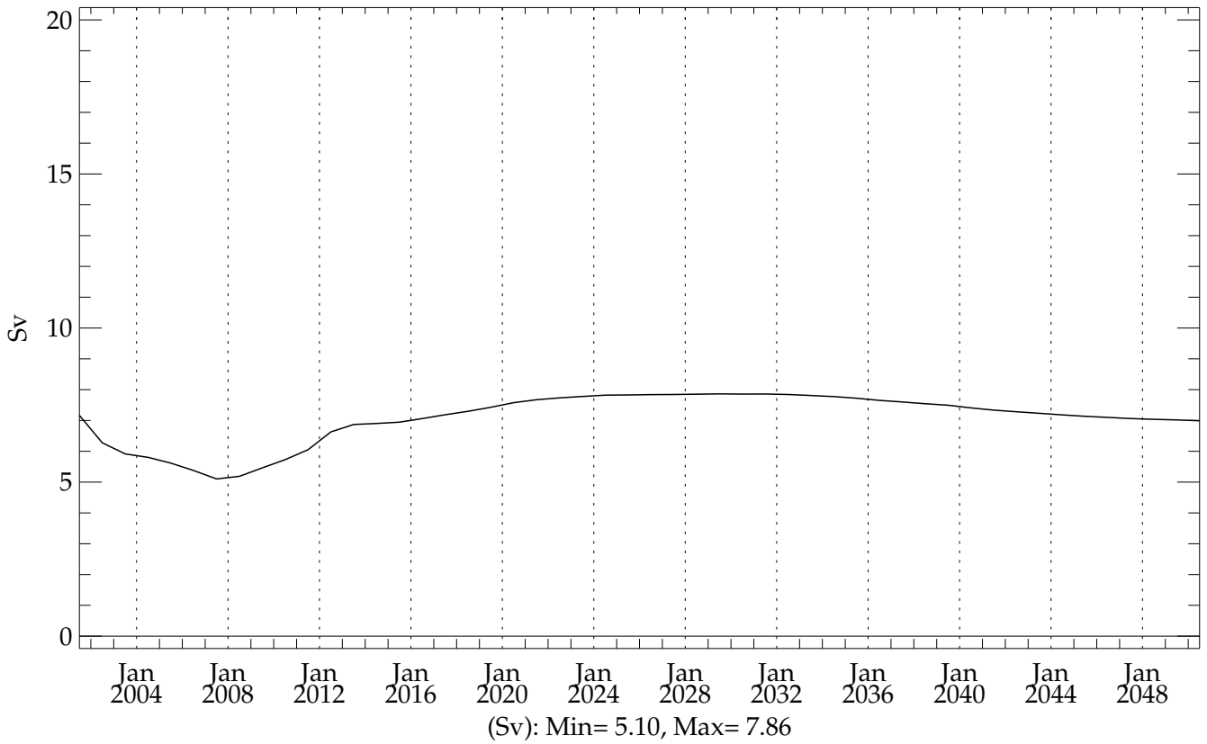
pstar4 (20010101 - 20501231) Max AntArctic Bottom Water between 80S and 65S (20010101 - 20501231)
