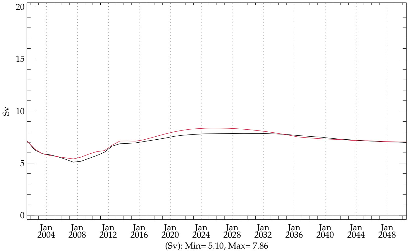
pstar4 (BLACK) - testht (RED) (20010101 - 20501231) Max AntArctic Bottom Water between 80S and 65S
