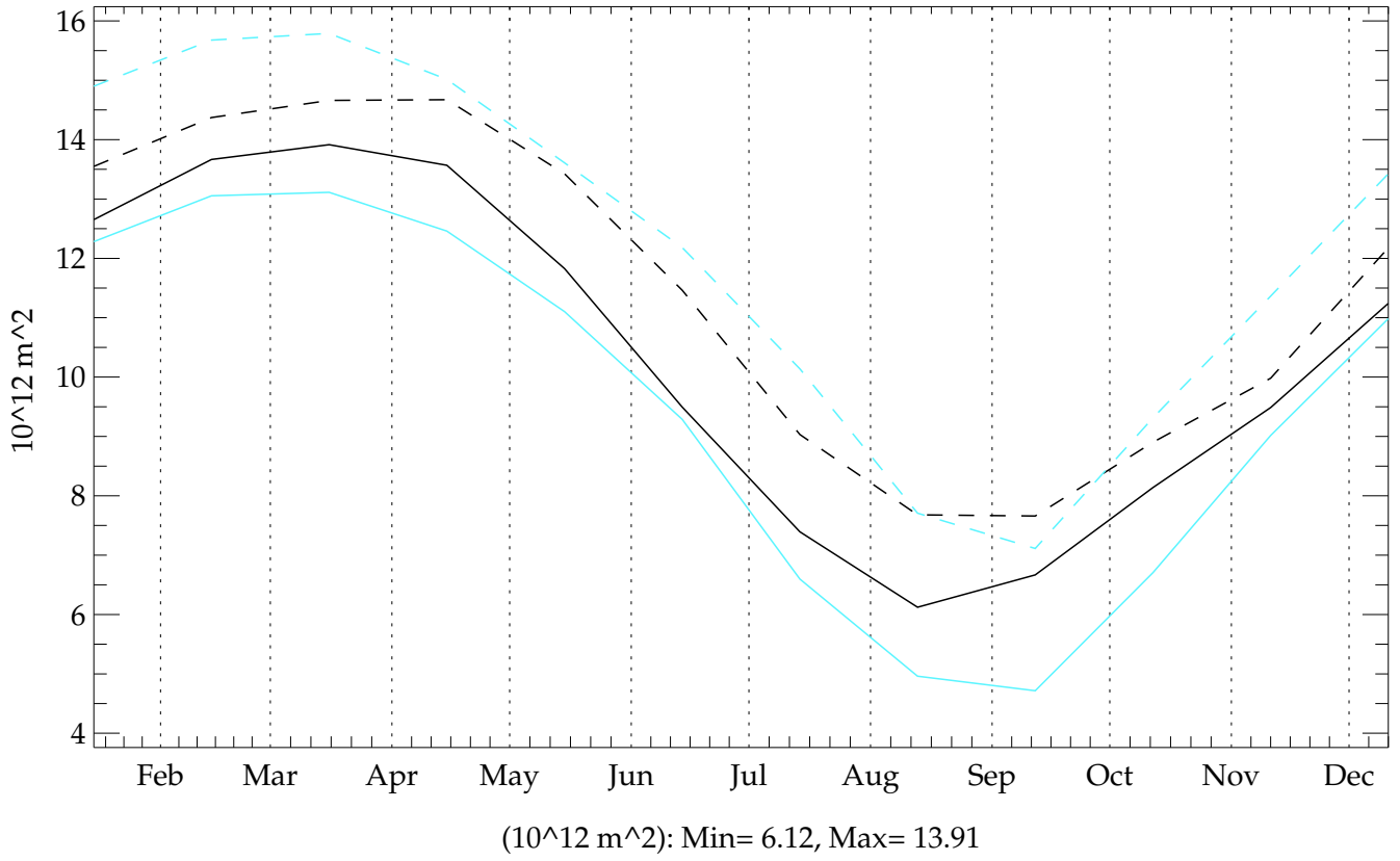
Southern Hemisphere pstar4 (BLACK) (20010101 - 20501231) OBSERVATION (light blue) Global Annual Mean Ice Area (CONTINUOUS) and Extend minus 15% (DASHED)
