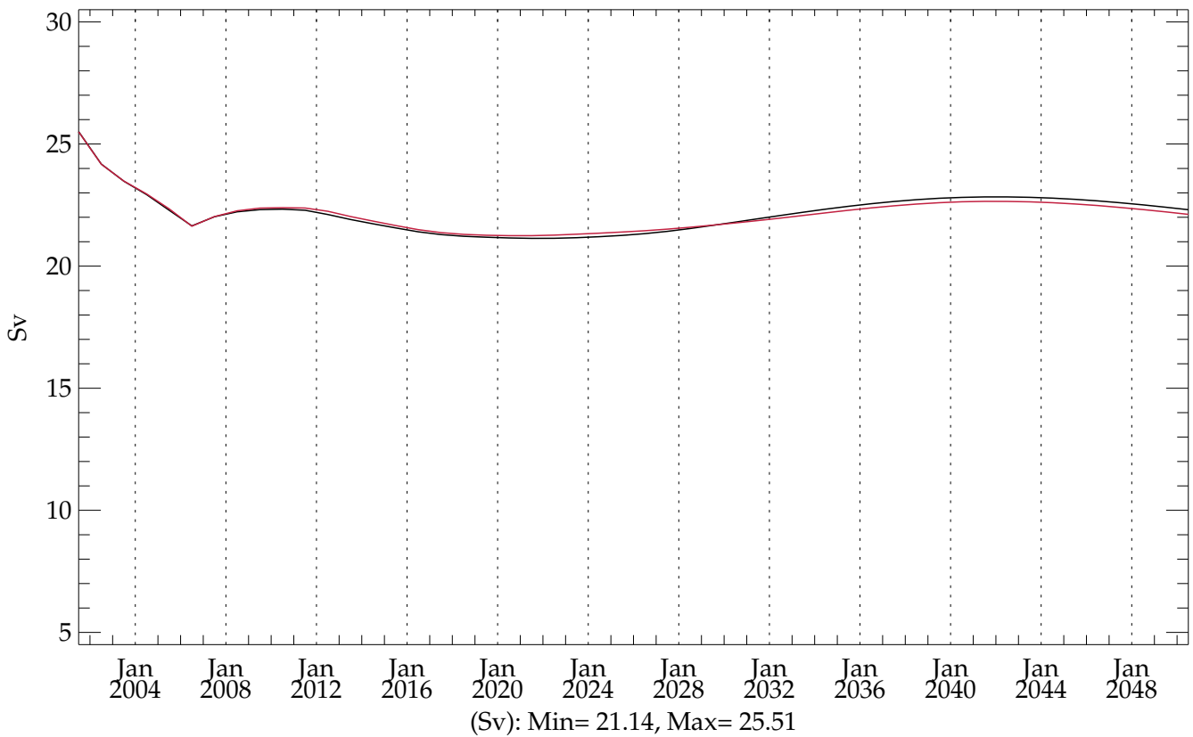
pstar4 (BLACK) - testht (RED) (20010101 - 20501231) Max AntArctic Bottom Cell between 65S and 30N
