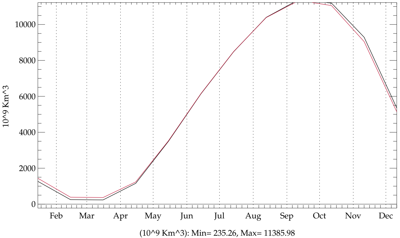
Southern Hemisphere pstar4 (BLACK) - testht (RED) (20010101 - 20501231) Global Annual Mean Ice Volume
