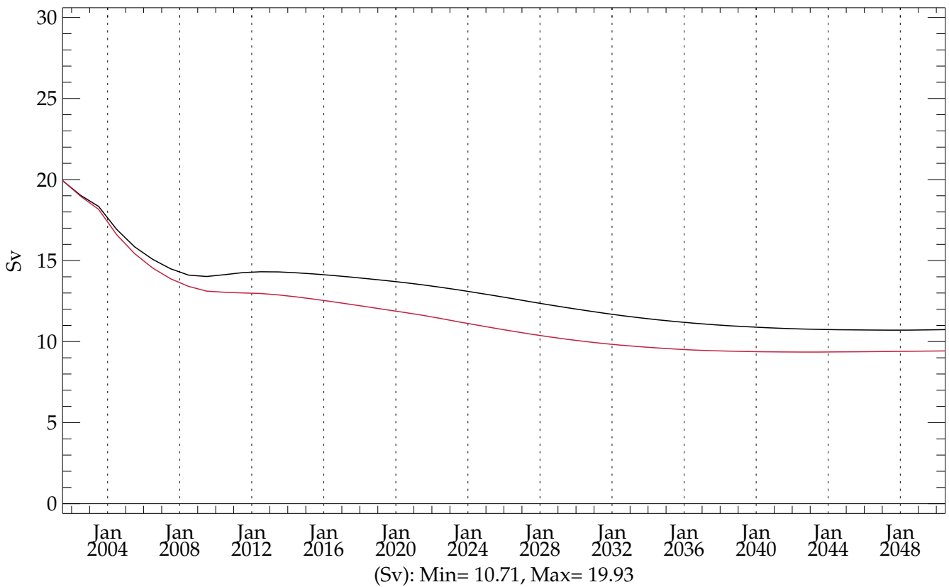
pstar4 (BLACK) - testht (RED) (20010101 - 20501231) Max Atlantic MOC between 40N and 50N
