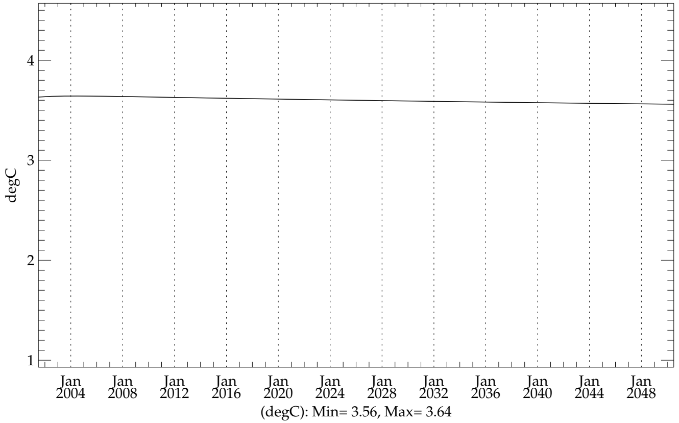
pstar4 (20010101 - 20501231) Global Mean Temperature
