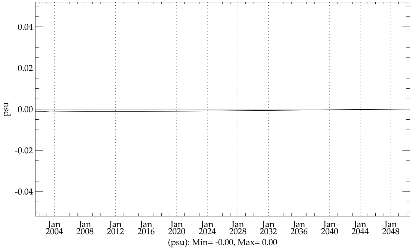
pstar4 (20010101 - 20501231) - Levitus Global Mean Salinity
