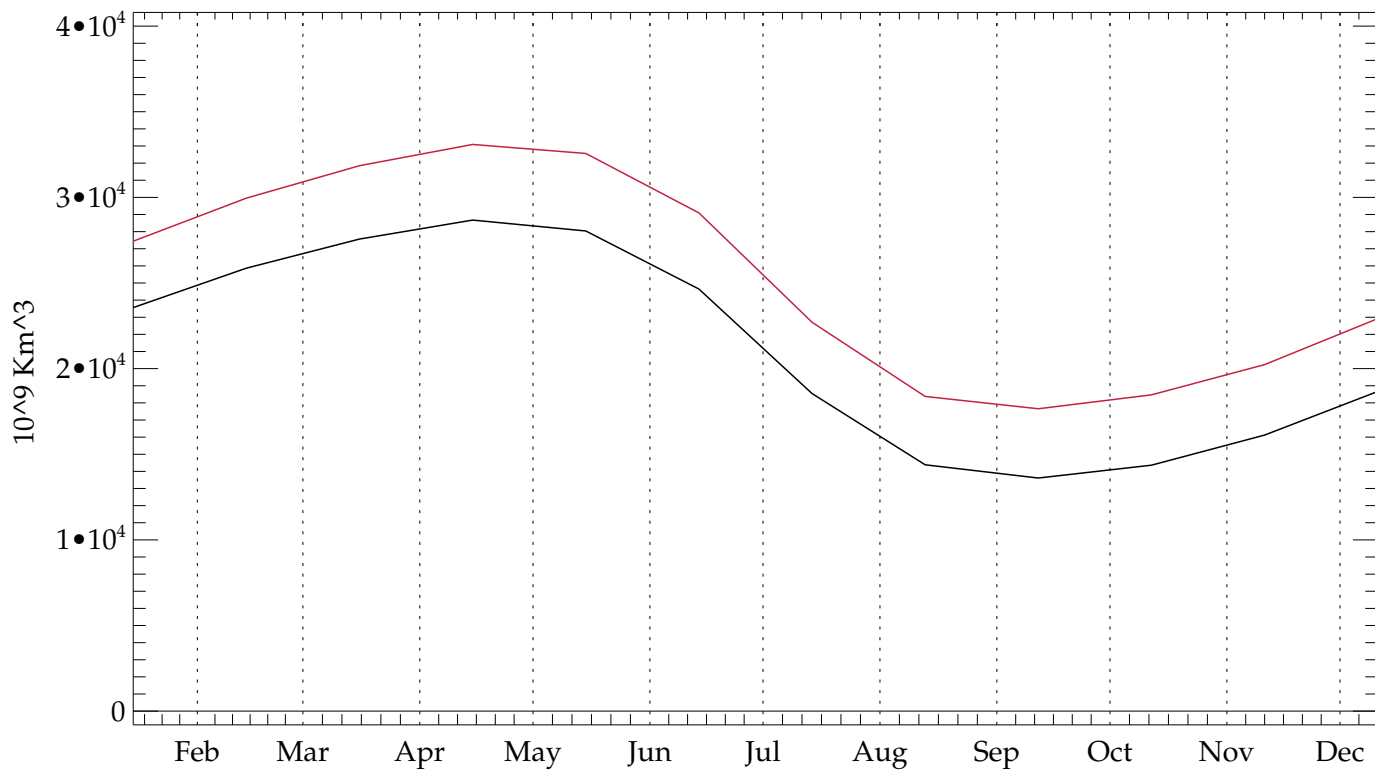
Northern Hemisphere c3p4h2a5 (BLACK) - htconv1 (RED) (20010101 - 20101231) Global Annual Mean Ice Volume (BLACK)
