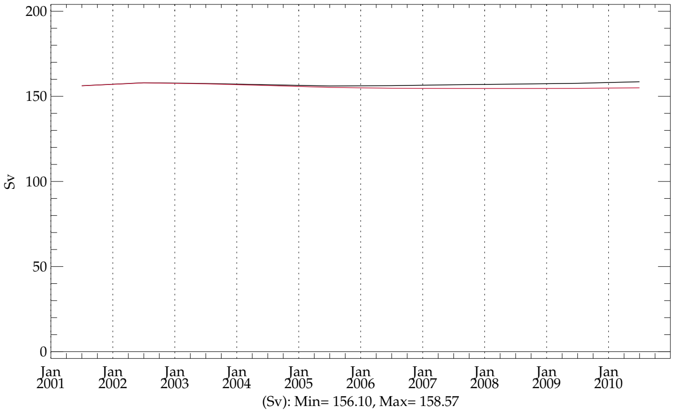
c3p4h2a5 (BLACK) - htconv1 (RED) (20010101 - 20101231) Drake Transport
