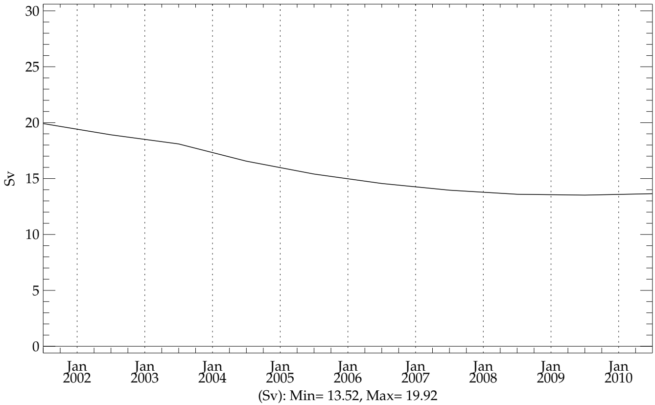
c3p4h2a5 (20010101 - 20101231) Max Atlantic MOC between 40N and 50N
