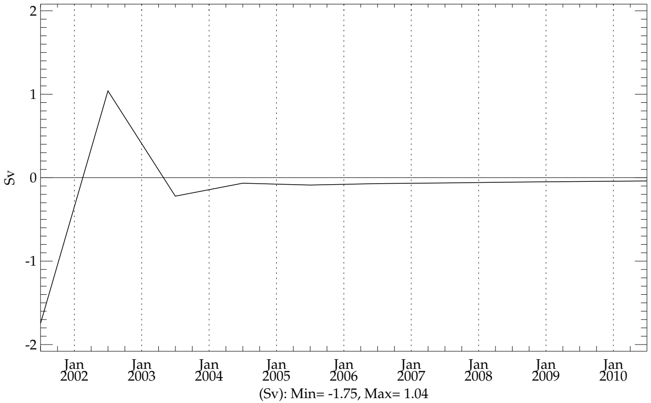
c3p4h2a5 (20010101 - 20101231) Global Mean EMP
