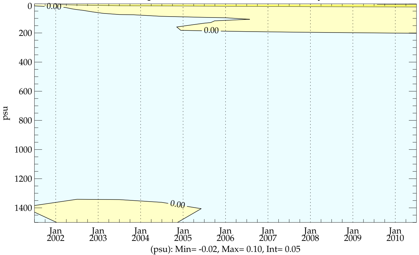
c3p4h2a5 (20010101 - 20101231) - Levitus ZT-plot (0-1500m) Global Mean Salinity
