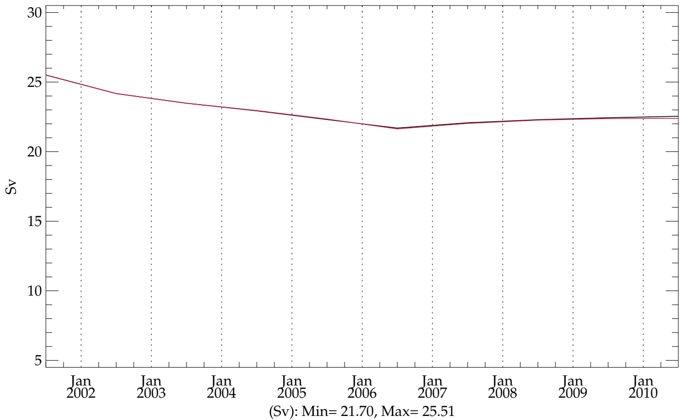
c3p4h2a5 (BLACK) - htconv1 (RED) (20010101 - 20101231) Max AntArctic Bottom Cell between 65S and 30N
