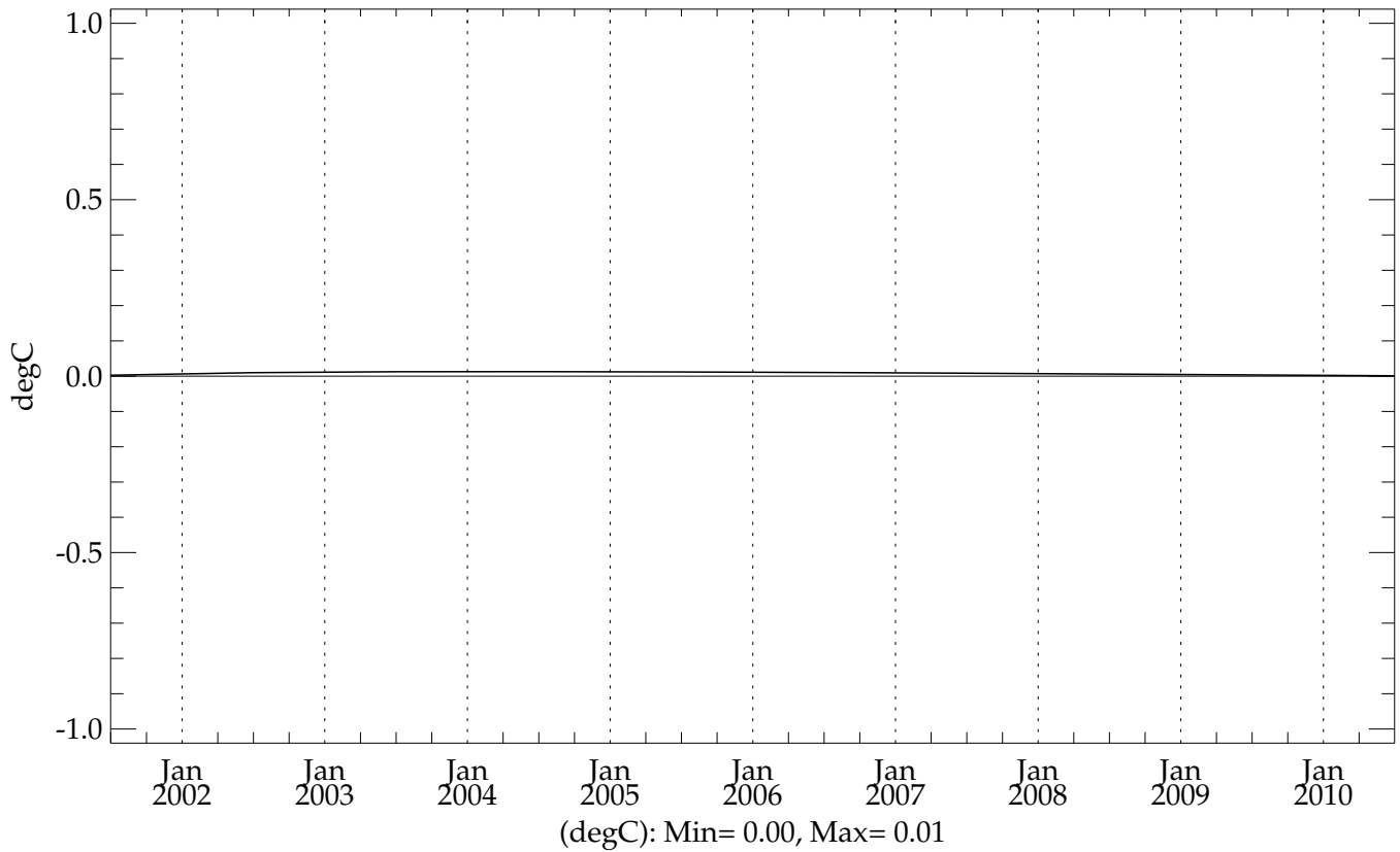
c3p4h2a5 (20010101 - 20101231) - Levitus Global Mean Temperature
