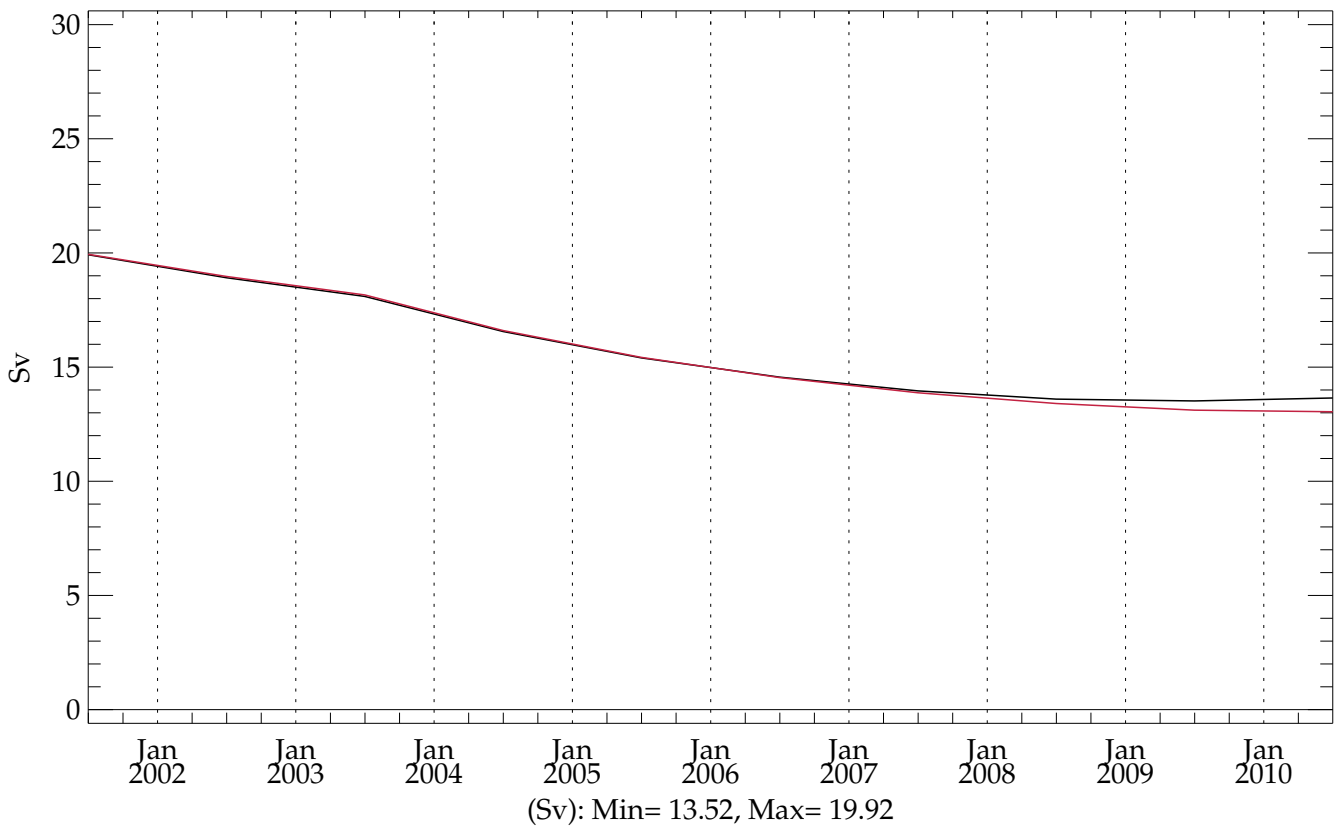
c3p4h2a5 (BLACK) - htconv1 (RED) (20010101 - 20101231) Max Atlantic MOC between 40N and 50N
