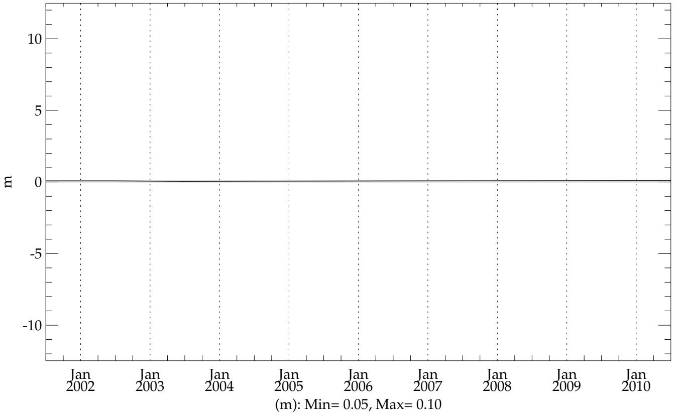
c3p4h2a5 (20010101 - 20101231) Global Mean SSH
