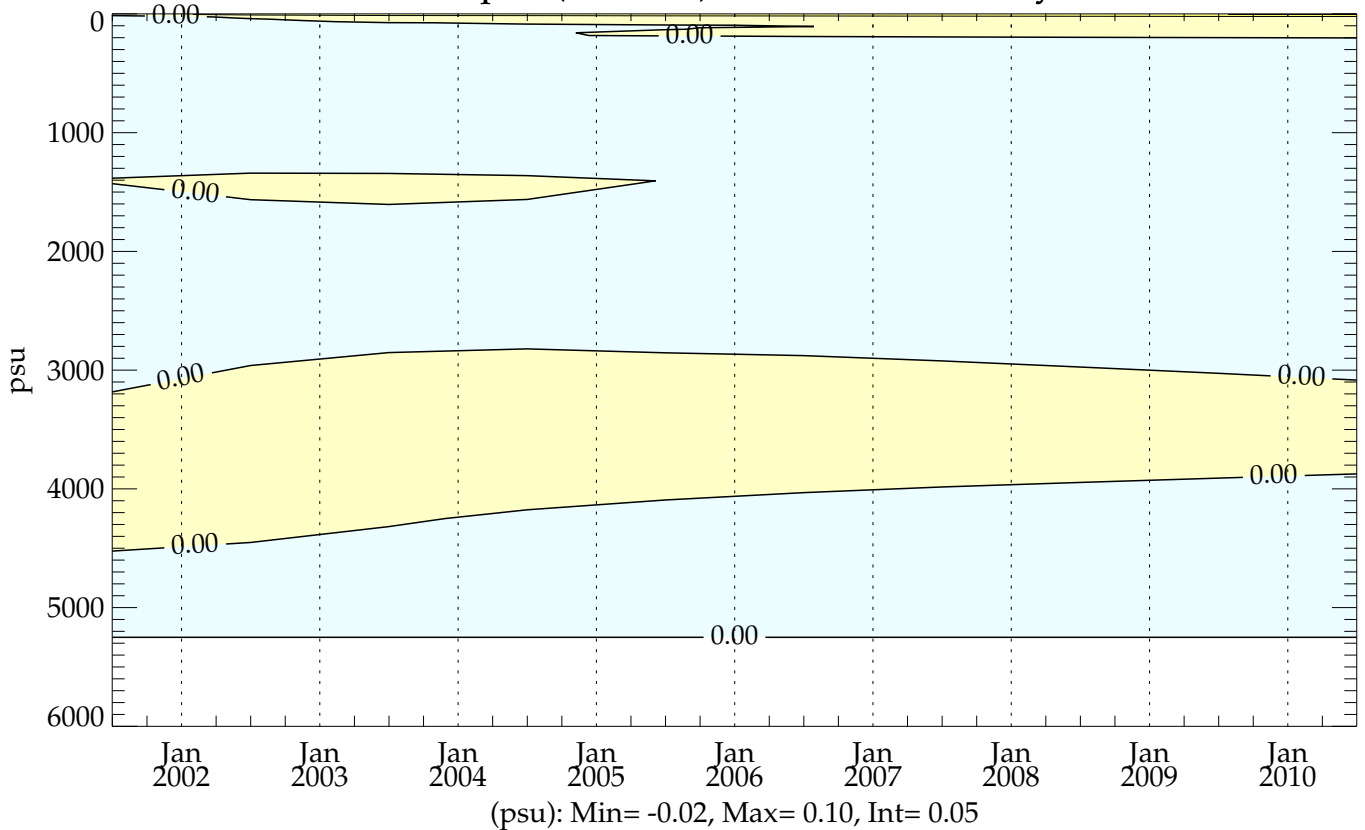
c3p4h2a5 (20010101 - 20101231) - Levitus ZT-plot (0-6000m) Global Mean Salinity
