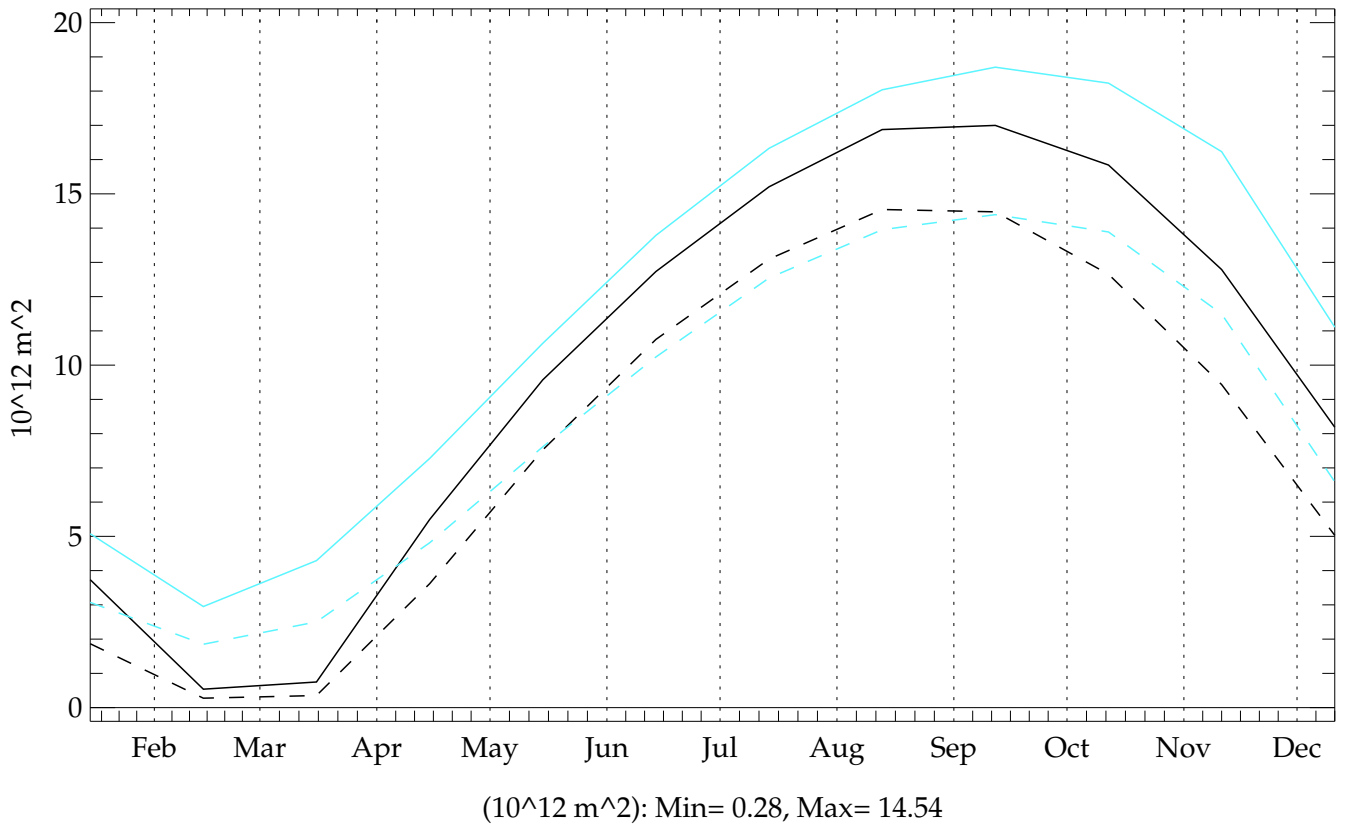
Southern Hemisphere c3p4h2a5 (BLACK) (20010101 - 20101231) OBSERVATION (light blue) Global Annual Mean Ice Area (DASHED) and Extend minus 15% (CONTINUOUS)
