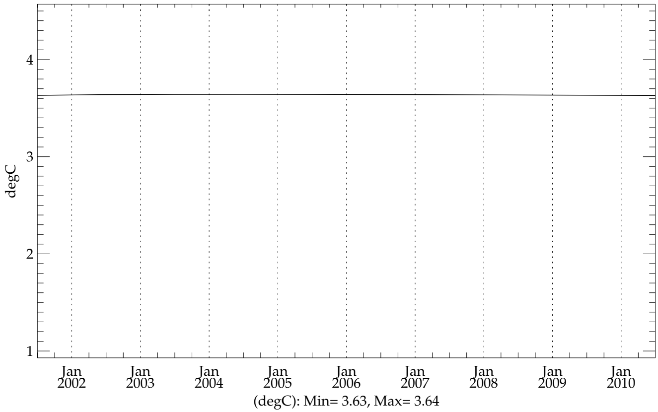
c3p4h2a5 (20010101 - 20101231) Global Mean Temperature
