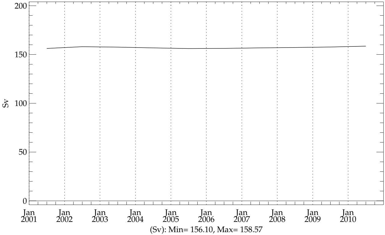
c3p4h2a5 (20010101 - 20101231) Drake Transport
