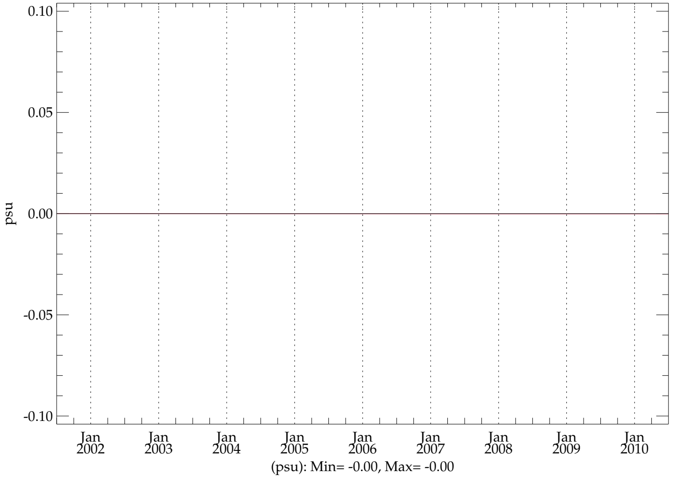
c3p4h2a5 - htconv1 (20010101 - 20101231) ZT-plot (0-6000m) Global Mean Salinity
