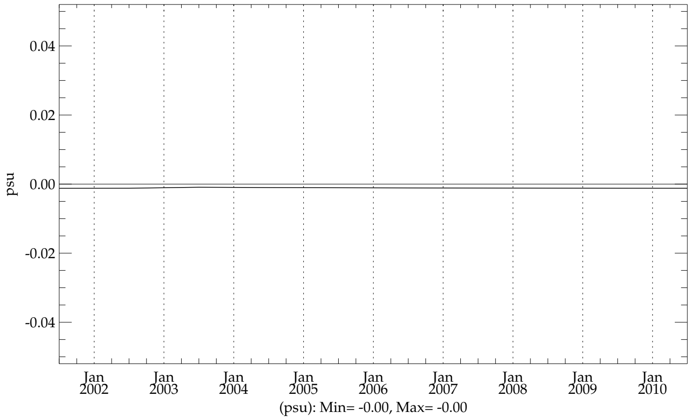
c3p4h2a5 (20010101 - 20101231) - Levitus Global Mean Salinity
