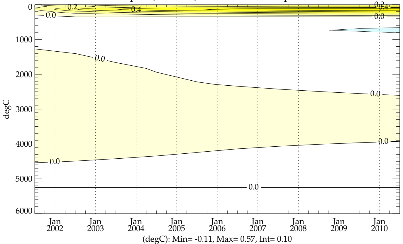
c3p4h2a5 (20010101 - 20101231) - Levitus ZT-plot (0-6000m) Global Mean Temperature
