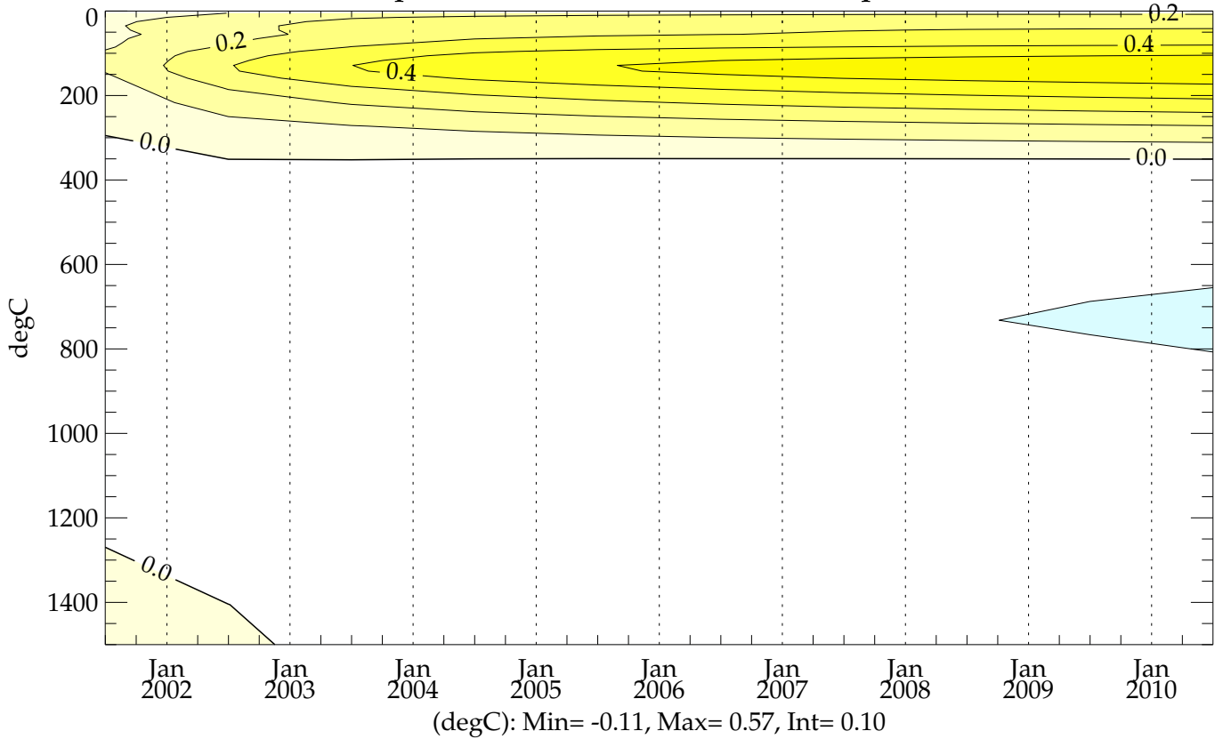
c3p4h2a5 (20010101 - 20101231) - Levitus ZT-plot (0-1500m) Global Mean Temperature
