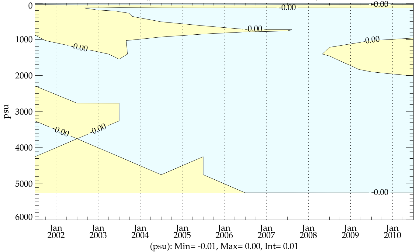
c3p4h2a5 - htconv1 (20010101 - 20101231) ZT-plot (0-6000m) Global Mean Salinity
