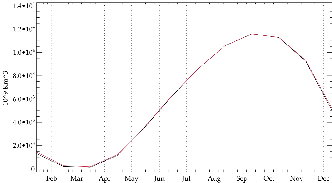
Southern Hemisphere c3p4h2a5 (BLACK) - htconv1 (RED) (20010101 - 20101231) Global Annual Mean Ice Volume
