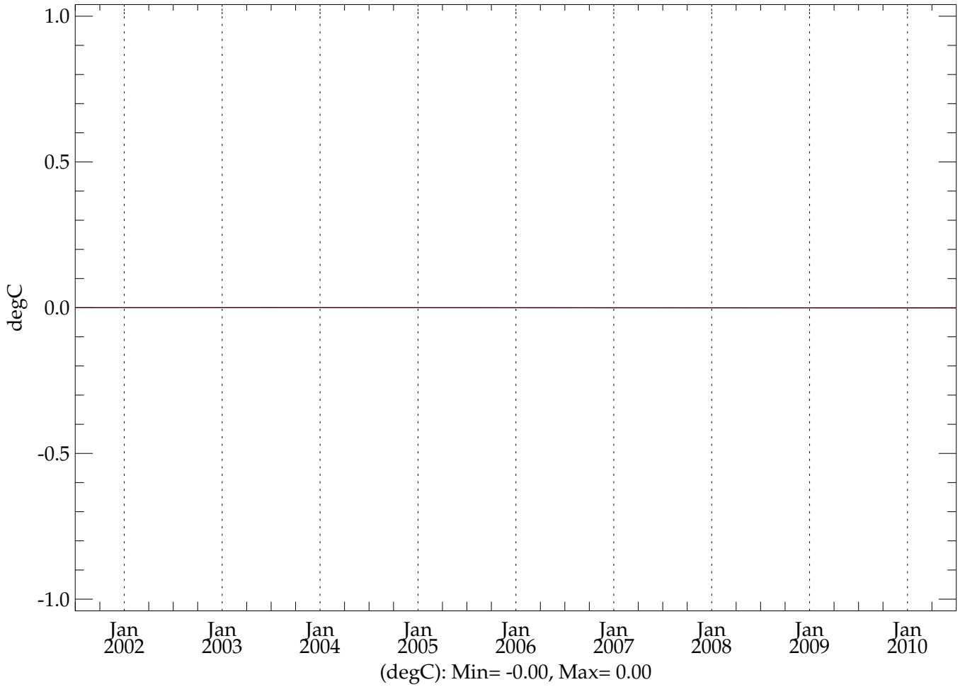
c3p4h2a5 - htconv1 (20010101 - 20101231) ZT-plot (0-6000m) Global Mean Temperature
