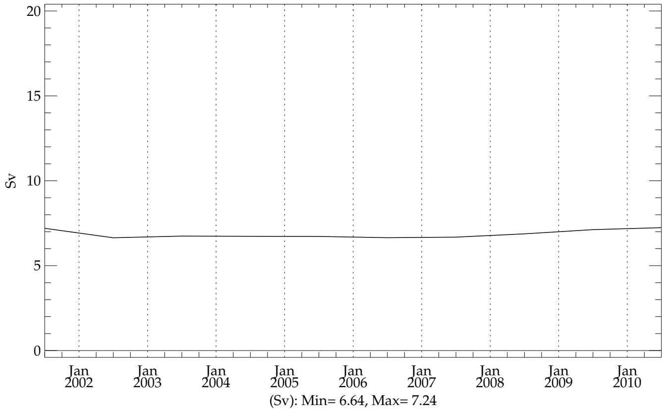
c3p4h2a5 (20010101 - 20101231) Max AntArctic Bottom Water between 80S and 65S (20010101 - 20101231)
