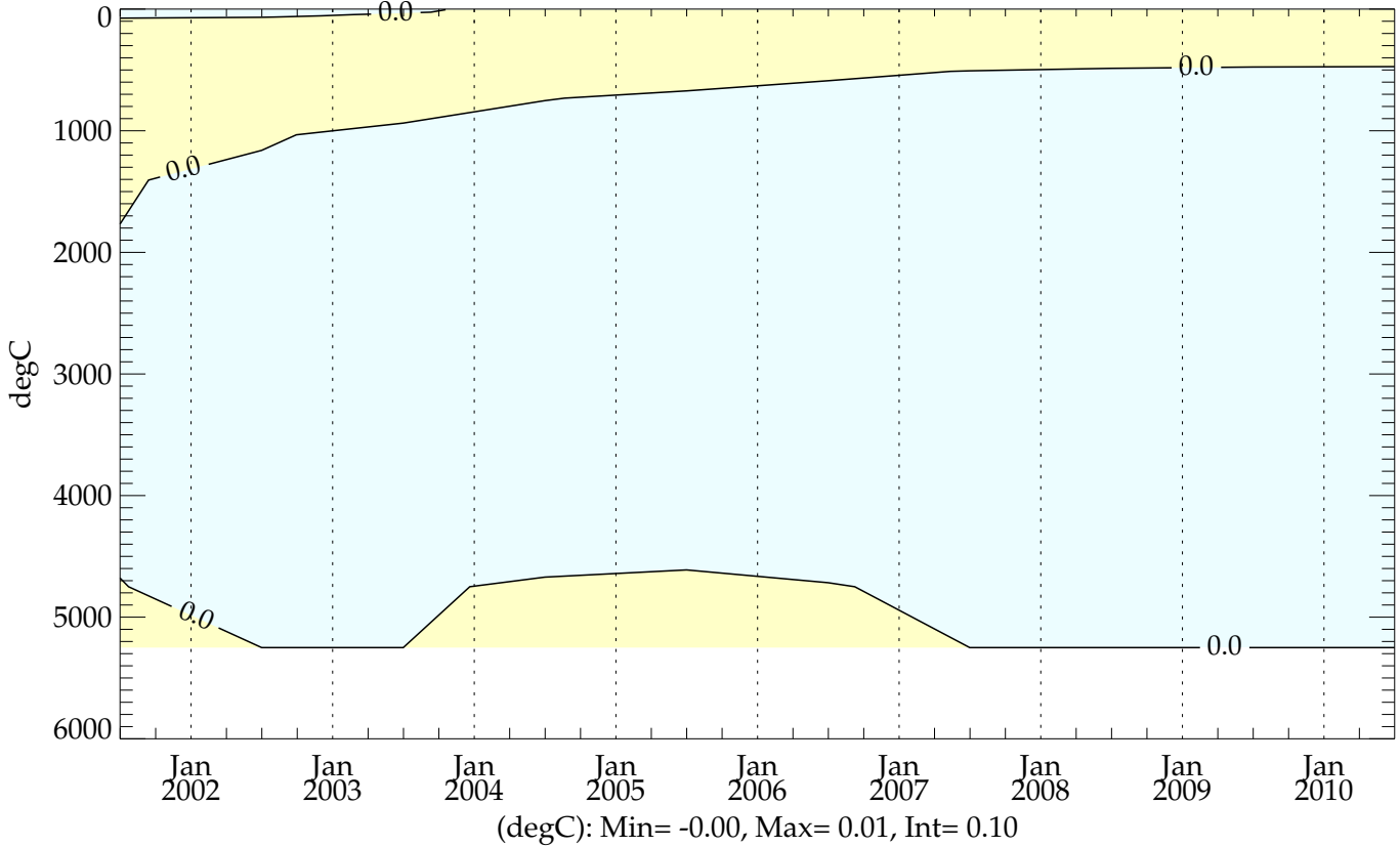
c3p4h2a5 - htconv1 (20010101 - 20101231) ZT-plot (0-6000m) Global Mean Temperature
