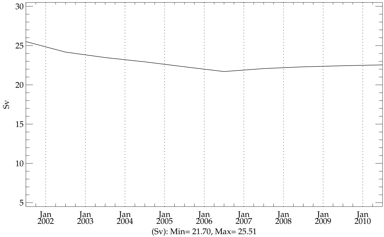
c3p4h2a5 (20010101 - 20101231) Max AntArctic Bottom Cell between 65S and 30N (20010101 - 20101231)
