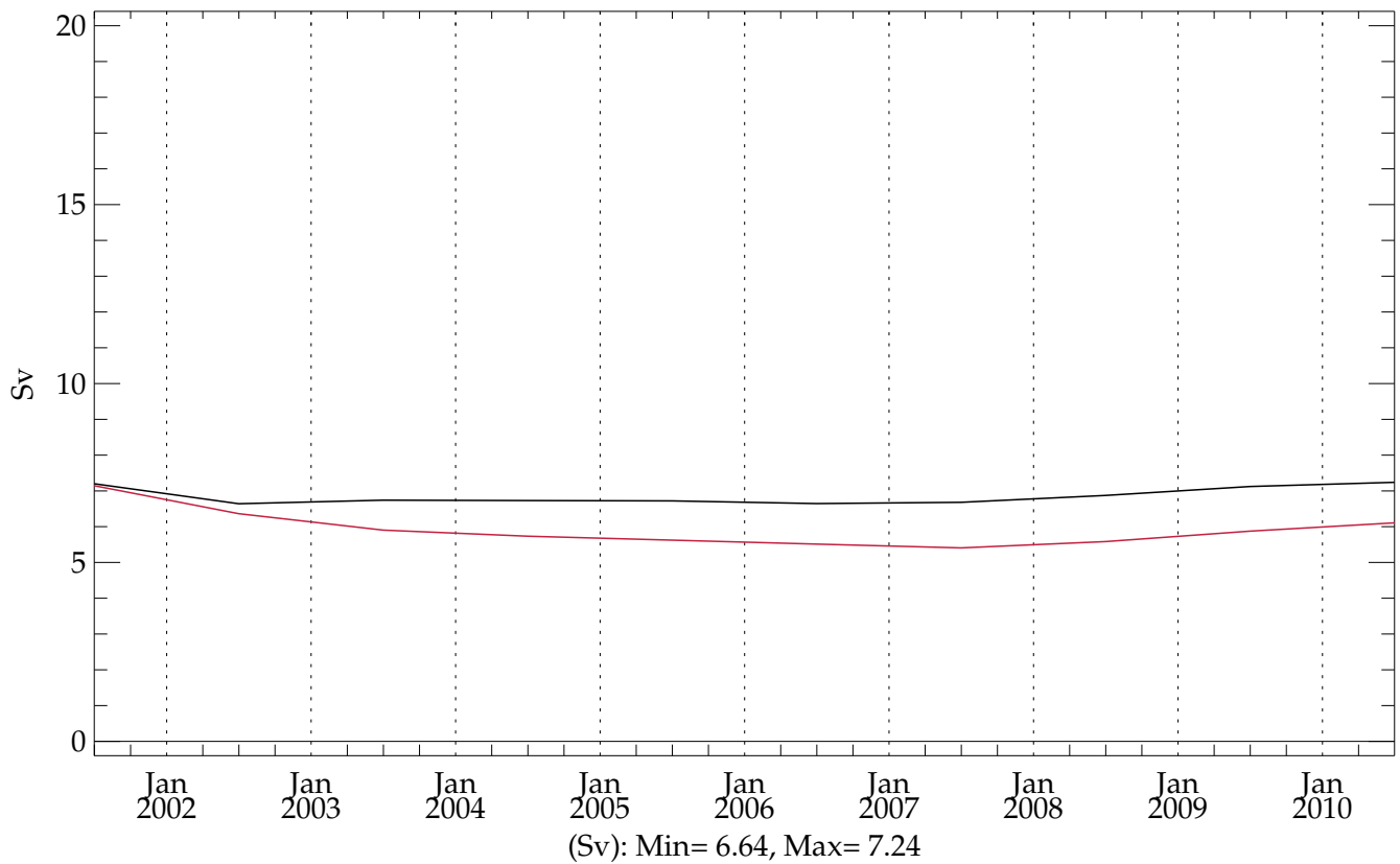
c3p4h2a5 (BLACK) - htconv1 (RED) (20010101 - 20101231) Max AntArctic Bottom Water between 80S and 65S
