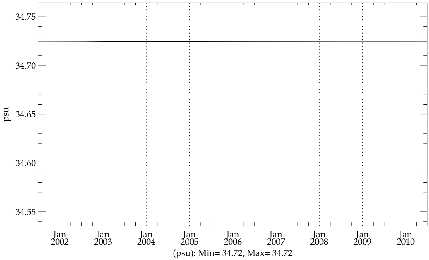
c3p4h2a5 (20010101 - 20101231) Global Mean Salinity
