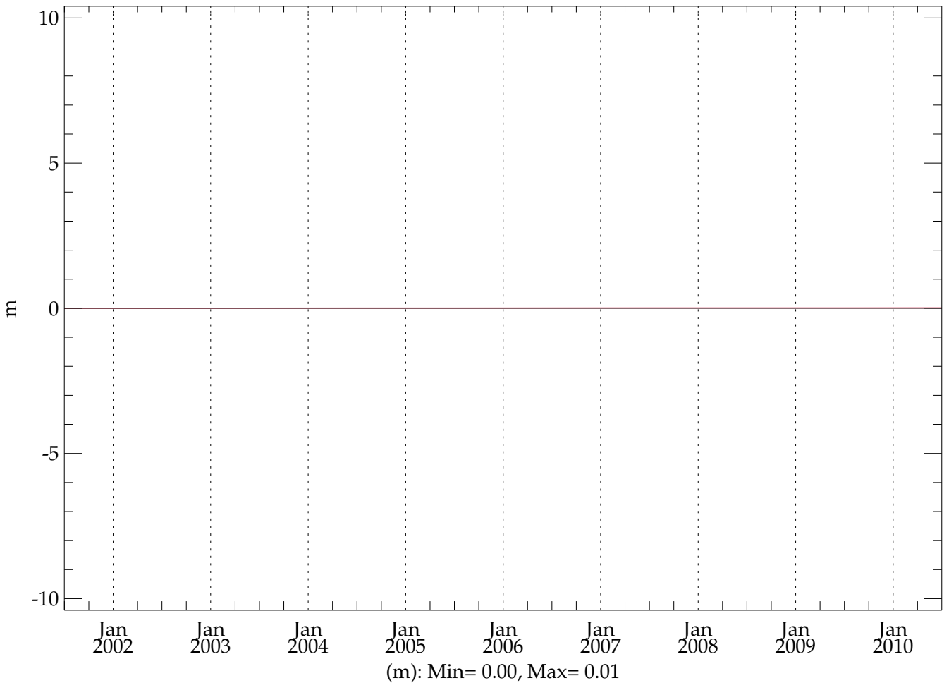
c3p4h2a5 (BLACK) - htconv1 (RED) (20010101 - 20101231) Global Mean SSH
