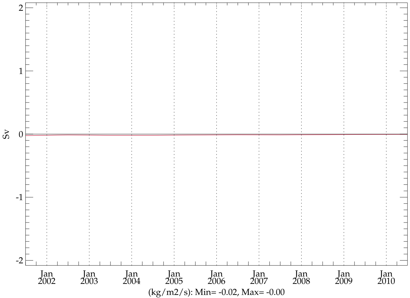
c3p4h2a5 (BLACK) - htconv1 (RED) (20010101 - 20101231) Global Mean EMP
