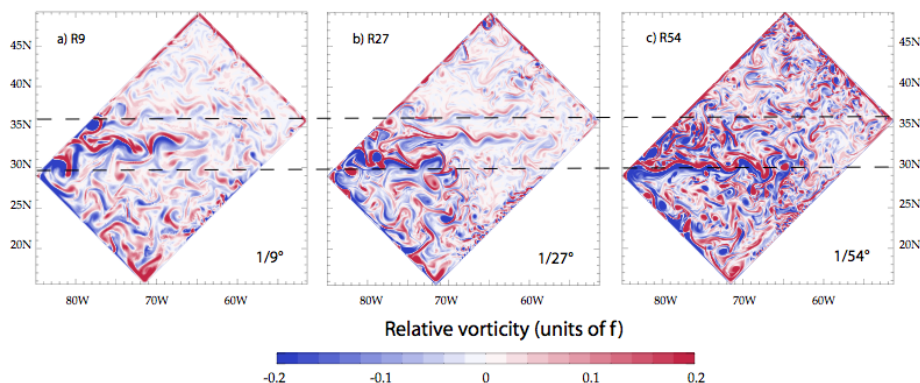
FIG. 16.3: Snapshot of relative vorticity at the surface of the model domain in GYRE R9, R27 and R54. From ?.
