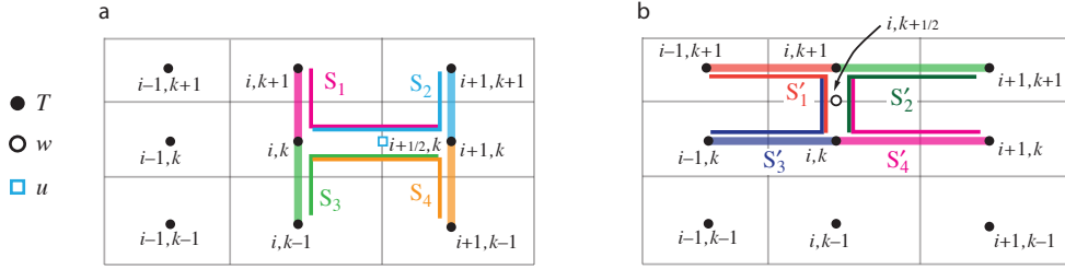
FIGURE D.1: (a) Arrangement of triads S_i and tracer gradients to give lateral tracer flux from box i, k to i + 1, k (b) Triads S'_i and tracer gradients to give vertical tracer flux from box i, k to i, k + 1 .
