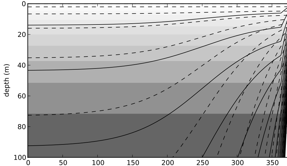
FIGURE 4.8: A comparison of the ? S -coordinate (solid lines), a 50 level Z -coordinate (contoured surfaces) and the ? S -coordinate (dashed lines) in the surface 100m for a idealised bathymetry that goes from 50m to 5500m depth. For clarity every third coordinate surface is shown.
