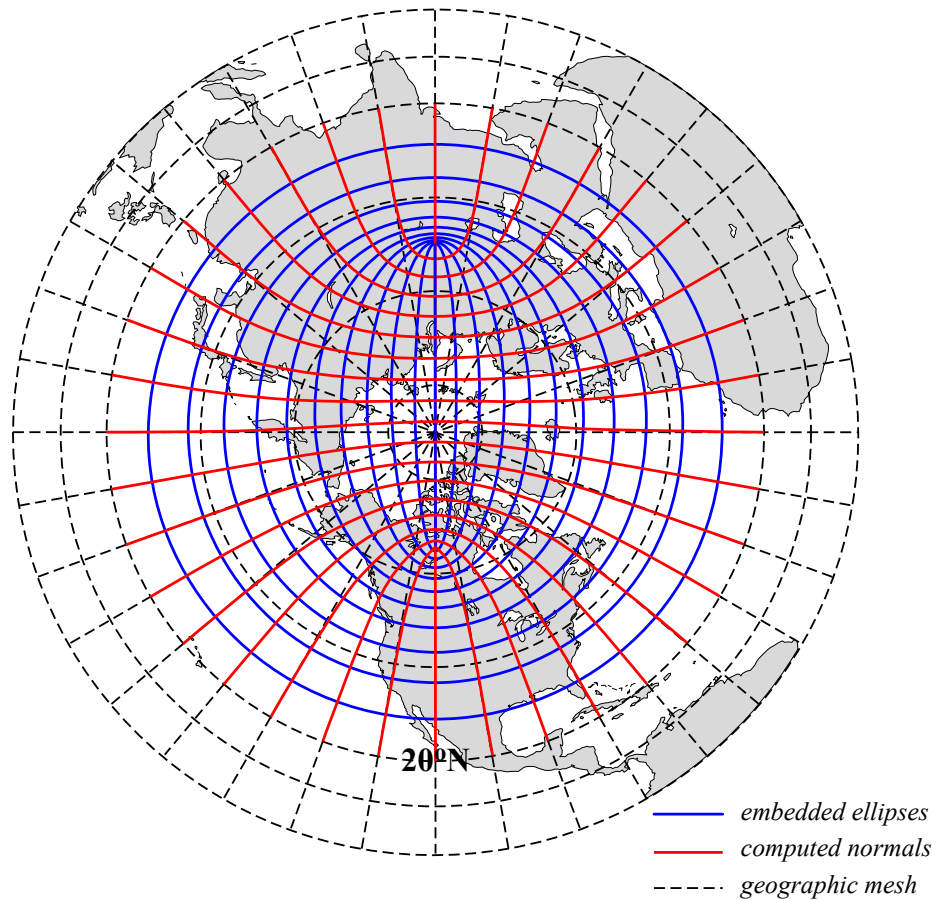
FIGURE 16.1: ORCA mesh conception. The departure from an isotropic Mercator grid start poleward of 20°N. The two "north pole" are the foci of a series of embedded ellipses (blue curves) which are determined analytically and form the i-lines of the ORCA mesh (pseudo latitudes). Then, following ?, the normal to the series of ellipses (red curves) is computed which provide the j-lines of the mesh (pseudo longitudes).
