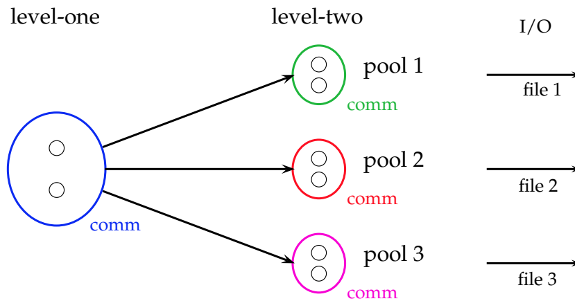
Figure 7.1: Two levels of servers for the total number of servers of 8 and \text{ratio\_server2}=75\% . The number of level-two servers is 8 \times \text{ratio\_server2} = 6 and, thus, the remaining 2 servers are of level one.
