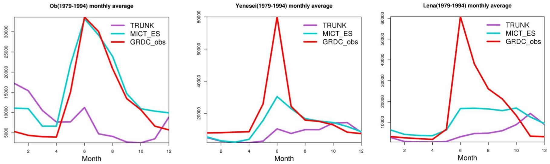
Figure 1: Streamflows observed (in red) and simulated at the mouth of the main Siberian rivers (in m^3/s ). The standard version of ORCHIDEE (Trunk) is plotted in purple and the new version (MICT_ES) including soil freezing and the improved snowpack model is plotted in cyan.
