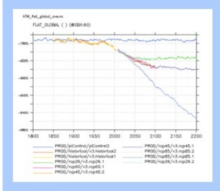
ATM_flat_global_ave
