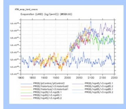
ATM_evap_land_ave
