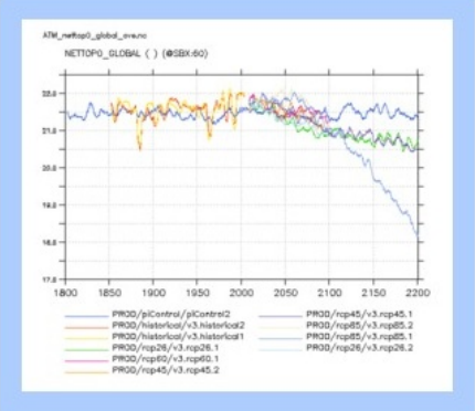
ATM_nettop0_global_ave
