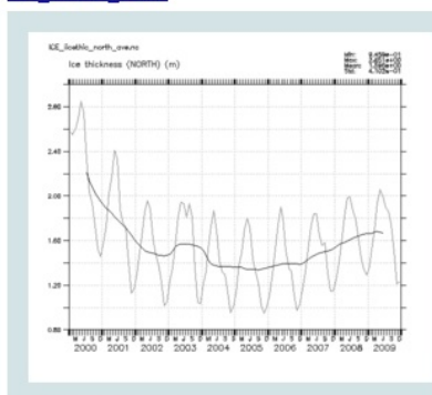
ICE_icethic_north
