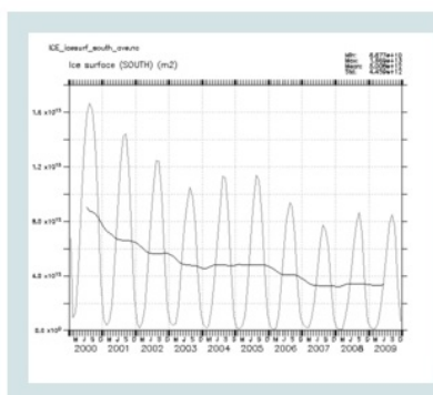
ICE_icesurf_south
