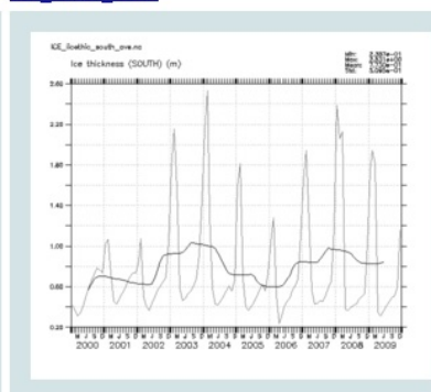
ICE_icethic_south
