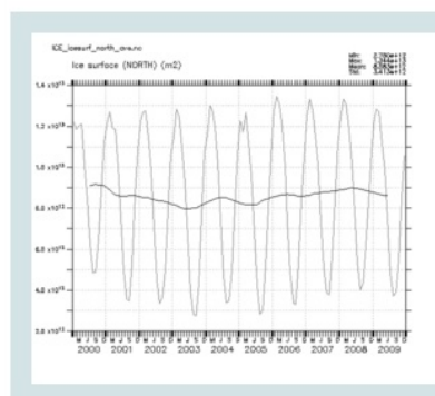
ICE_icesurf_north
