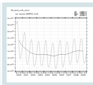
ICE_icevol_north
