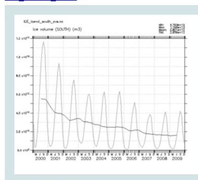
ICE_icevol_south
