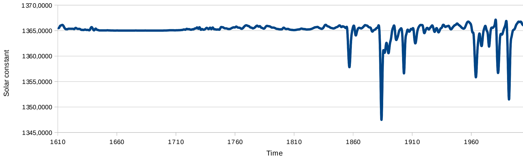
Annual solar constant evolution (Solar & volcanoes)
