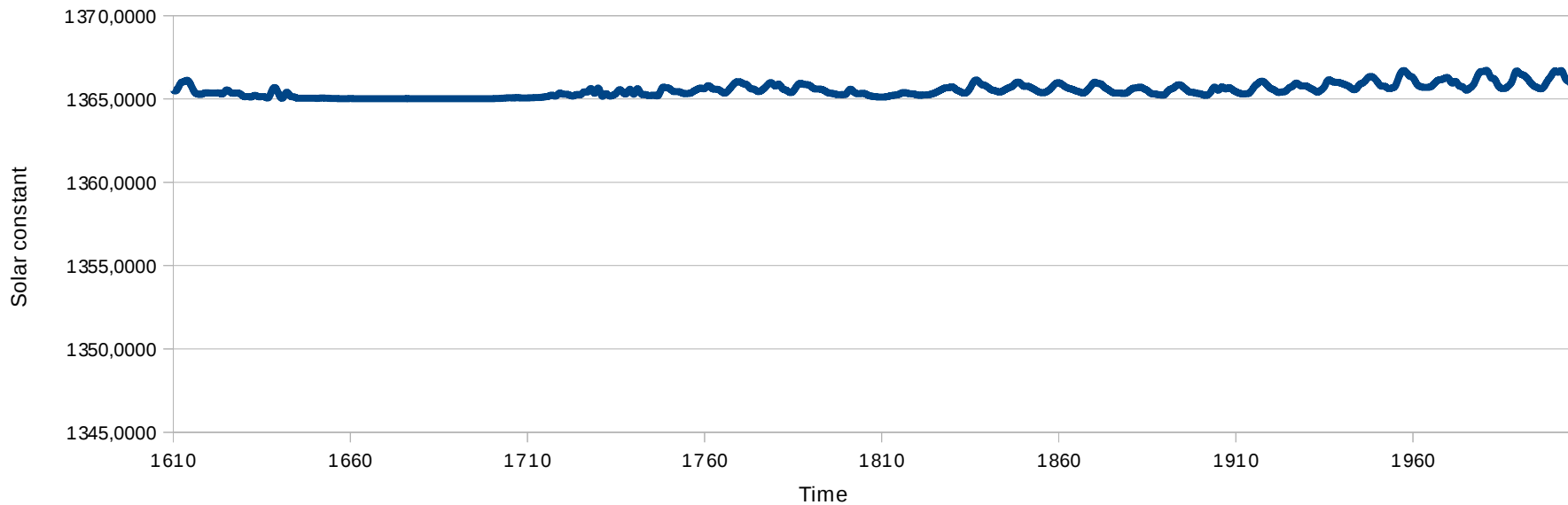
Annual solar constant evolution
