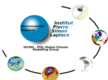
ATM_flat_global_ave
