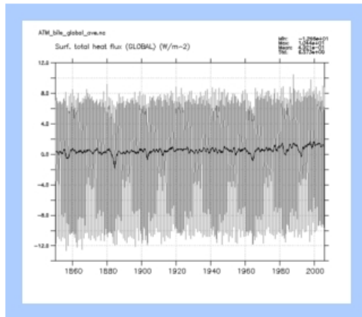
ATM_bils_global
