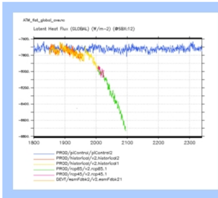
ATM_flat_global_ave
