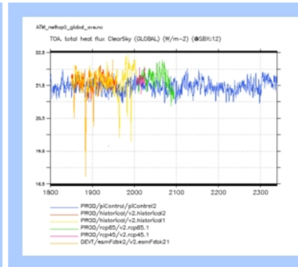
ATM_nettop0_global_ave
