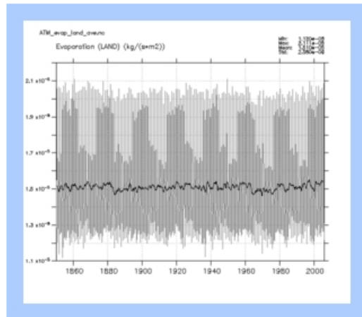
ATM_evap_land
