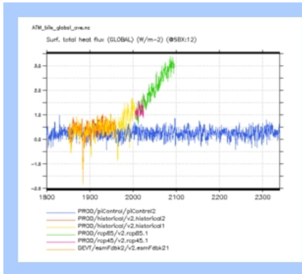
ATM_bils_global_ave
