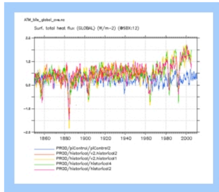
ATM_bils_global_ave
