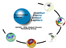
ATM_flat_global_ave
