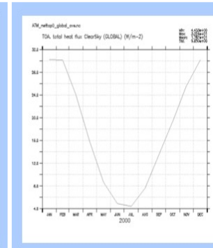
ATM_nettop0_global
