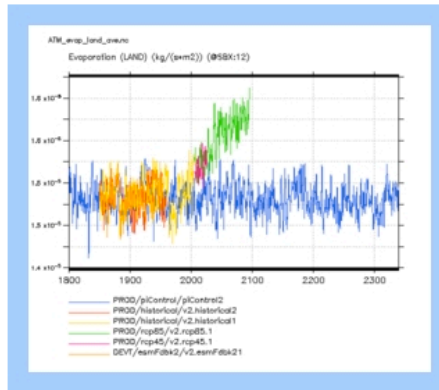
ATM_evap_land_ave
