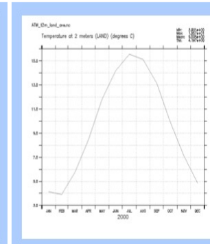
ATM_t2m_land
