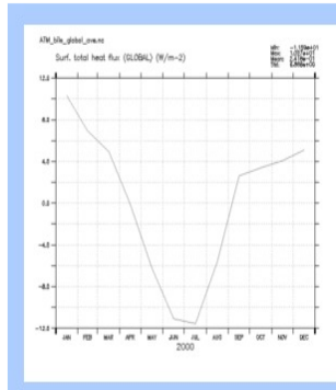
ATM_bils_global
