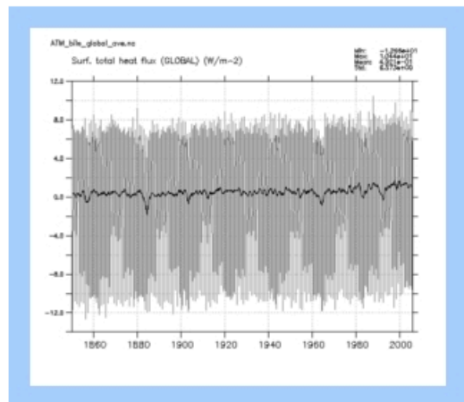
ATM_bils_global
