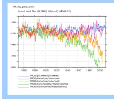
ATM_flat_global_ave
