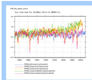
ATM_bils_global_ave
