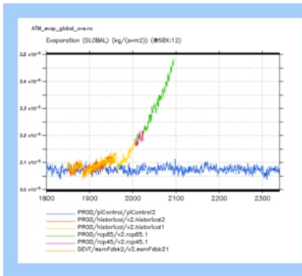
ATM_evap_global_ave
