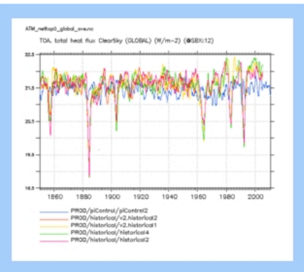
ATM_nettop0_global_ave
