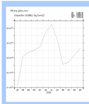
ATM_evap_global
