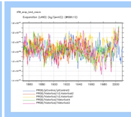
ATM_evap_land_ave
