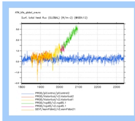
ATM_bils_global_ave
