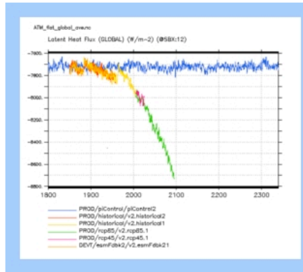
ATM_flat_global_ave
