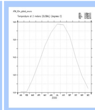
ATM_t2m_global
