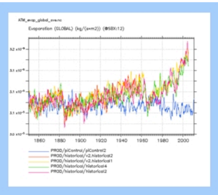
ATM_evap_global_ave
