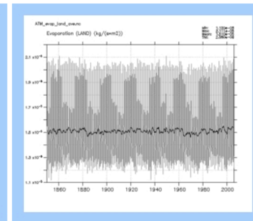
ATM_evap_land
