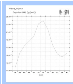
ATM_evap_land
