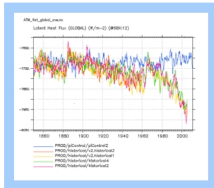
ATM_flat_global_ave
