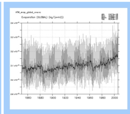
ATM_evap_global
