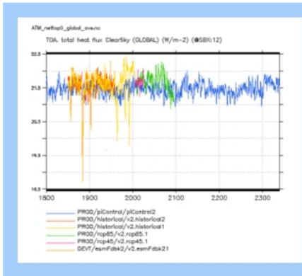
ATM_nettop0_global_ave
